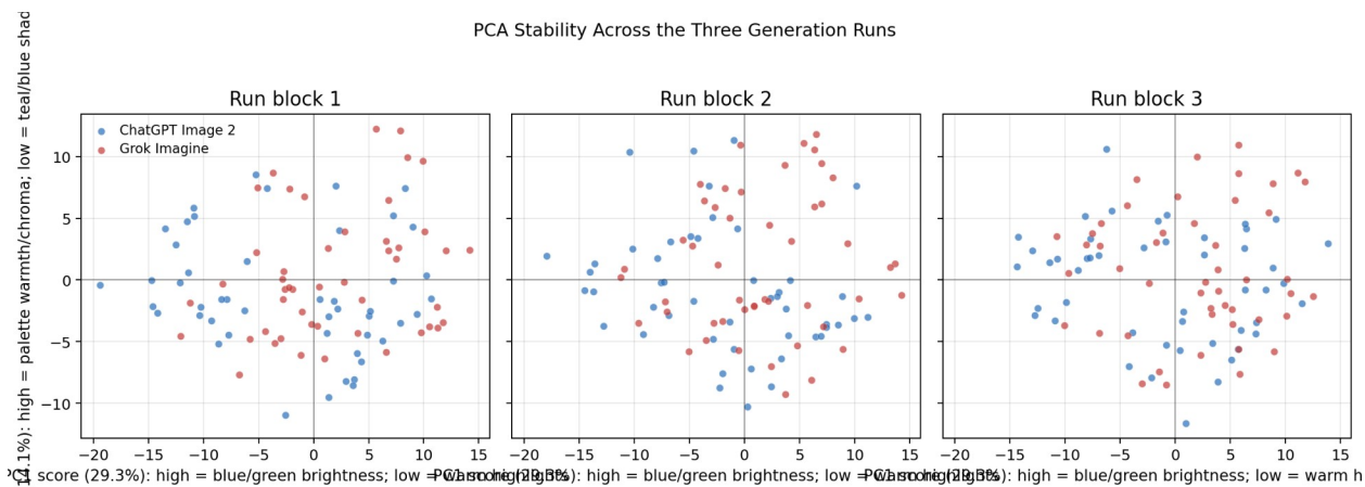
Appendix Figure A2. PCA by run block. The run blocks do not erase the main prompt structure.
