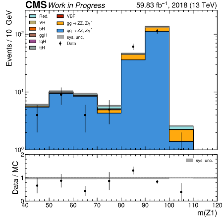
(b) Mass of the Z_1 candidate.
