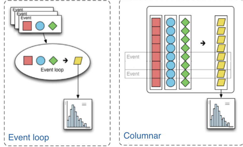
Figure 1: A representation of event loop based and columnar based analysis approaches can be seen on the left and right respectively [71]. The squares, circles and diamonds represent event data that is transformed via an algorithm into output that is histogrammed, represented by the trapezoids.
