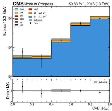
(f) CvsB discriminator of the selected jet.
