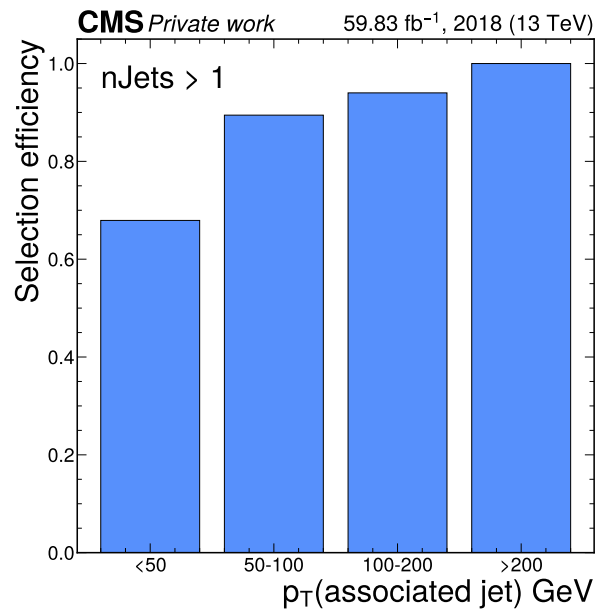
Figure 3.1: The efficiency with which the jet associated with the Higgs boson is selected via the described algorithm in simulated cH(ZZ \rightarrow 4\mu) events. This efficiency is shown in bins of the associated jet's transverse momentum for events in which more than one jet passes the jet selection requirements.
