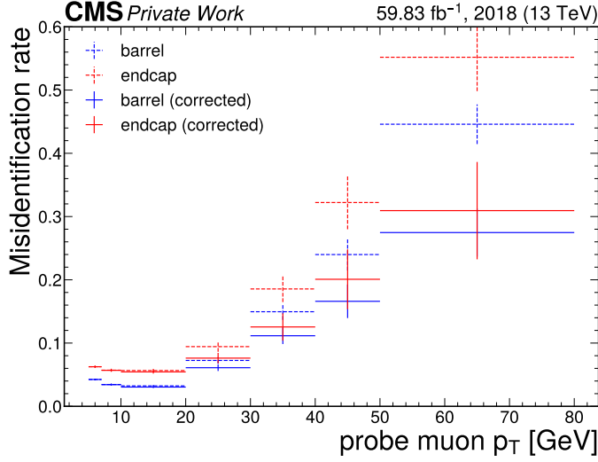
Figure 3.6: The muon misidentification rate in bins of the probe muon transverse momentum in both the barrel and endcap regions. The dotted lines represent the uncorrected misidentification rate while the solid lines represent the misidentification rate where contributions from WZ \rightarrow 3\ell\nu processes are subtracted.
