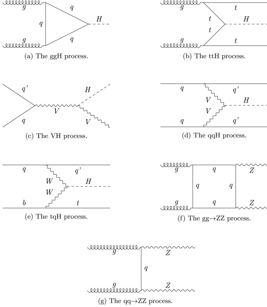
Figure 3.4: Representative Feynman diagrams of the irreducible background processes relevant to the cH(ZZ \rightarrow 4\mu) analysis. This includes the ggH , ttH , VH , qqH , tqH , gg \rightarrow ZZ and qq \rightarrow ZZ processes. When no final state parton is explicitly present in the diagram it is implied via, for example, parton radiation.
