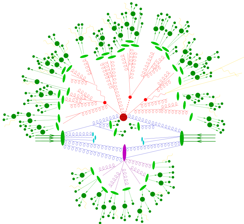
Figure 3.12: An overview of what an event simulation may look like [67]. The initial state particles originating from the protons are shown in blue. The hard scattering process is represented in red. Additional, soft scatterings are represented in purple. The hadronisation to form colourless hadrons (represented by dark green circles) is represented by the light green ellipses. Additional photon radiation is represented in yellow.
