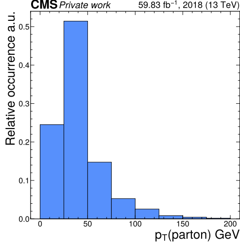
Figure 2.3: Transverse momentum of the parton produced alongside a Higgs boson in a Madgraph5_aMC@NLO [19] simulation of the cH process within the CMS detector, which typically takes on very small values. Since jets at very low transverse momenta cannot be well reconstructed in experiments such as the CMS detector, a minimum p_T requirement is introduced in the simulation to limit the simulation of events that are not expected to be experimentally accessible. This results in the appearance of a peak in the [25, 50] GeV bin of the distribution.
