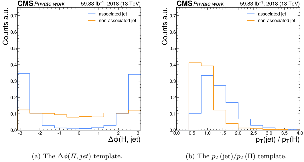
Figure 6: The \Delta\phi(H, jet) and p_T(jet)/p_T(H) templates in the 15-30 GeV bin of the Higgs candidate mass.
