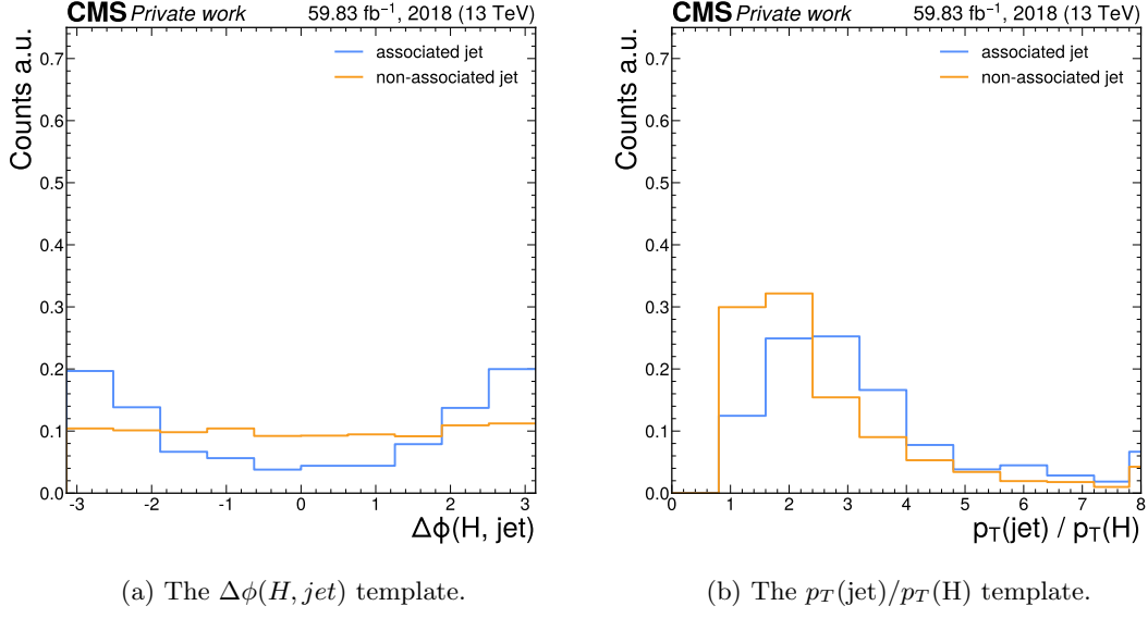
Figure 5: The \Delta\phi(H, jet) and p_T(jet)/p_T(H) templates in the 0-15 GeV bin of the Higgs candidate mass.
