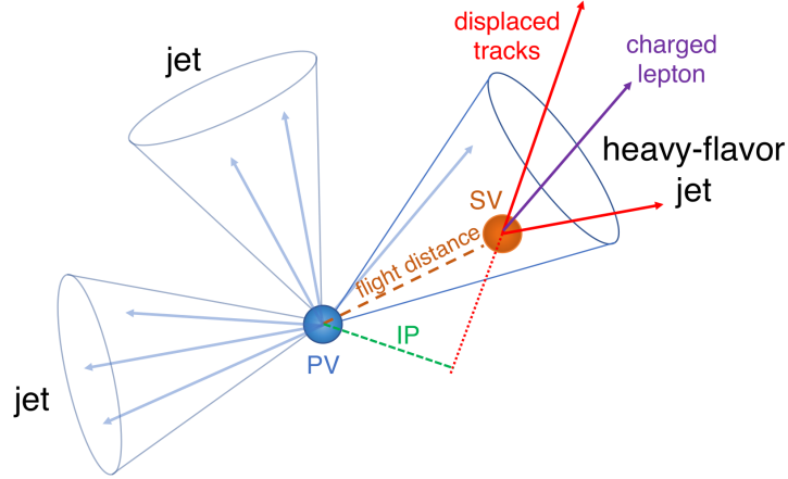
Figure 3.8: An illustration highlighting the properties of HF jets [55]. The presence of a secondary vertex (SV), characterised by the impact parameter (IP) in green, as well as the presence of a lepton is highlighted.
