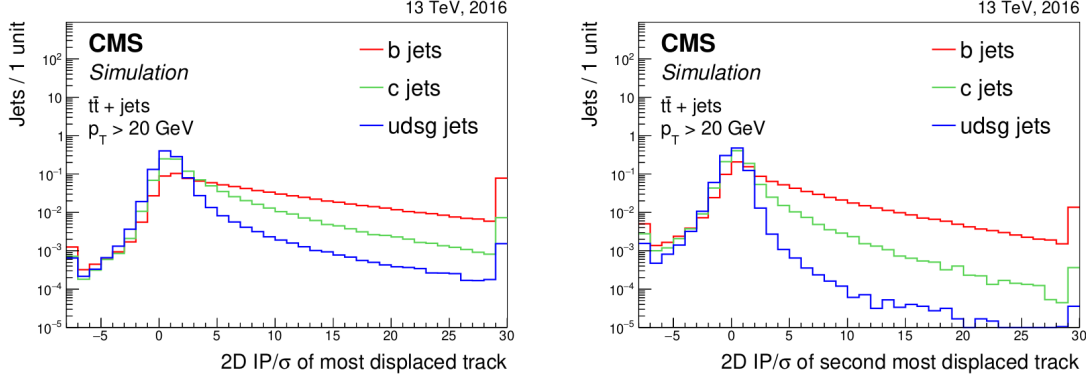
Figure 3.9: Plots showing the significance of the 2D impact parameter of the most and second most displaced tracks in a jet [55]. As can be seen, these variables can differentiate b and c jets from light jets to a significant degree.
