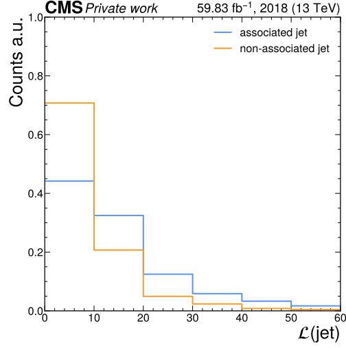
Figure 4.3: The distribution of the jet selection likelihood \mathcal{L}(\text{jet}) , in simulated cH(ZZ \rightarrow 4\mu) events in which an associated jet can be identified via a parton-to-jet matching, for associated and non-associated jets. It can be seen that on average, applying the jet selection algorithm on the associated jet produces a higher likelihood value than on non-associated jets, as expected.
