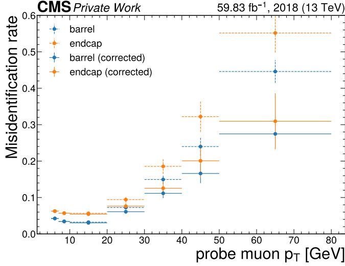
Figure 4.10: The muon misidentification rate in bins of the probe muon transverse momentum in both the barrel and endcap regions. The dotted lines represent the uncorrected misidentification rate while the solid lines represent the misidentification rate where contributions from WZ \rightarrow 3\ell\nu processes are subtracted.
