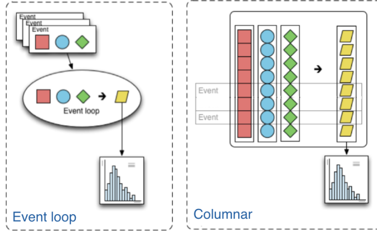
Figure 4: A representation of event loop based and columnar based analysis approaches can be seen on the left and right respectively [87]. The squares, circles and diamonds represent event data that is transformed via an algorithm into output that is histogrammed, represented by the trapezoids.
