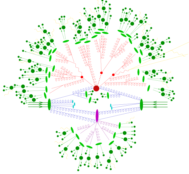
Figure 3.12: An overview of what an event simulation may look like [66]. The initial state particles originating from the protons are shown in blue. The hard scattering process is represented in red. Additional, soft scatterings are represented in purple. The hadronisation to form colourless hadrons (represented by dark green circles) is represented by the light green ellipses. Additional photon radiation is represented in yellow.
