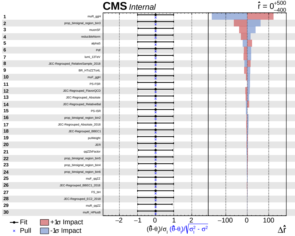
Figure 16: The 30 leading uncertainty sources in a fit of \sigma \mathcal{B}(\text{cH}(\text{ZZ} \rightarrow 4\mu))_{\kappa_c} with r = 0 , ordered by their relative impact on the fitted signal strength.
