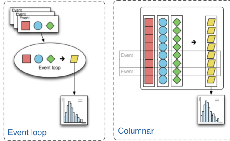
Figure 4: A representation of event loop based and columnar based analysis approaches can be seen on the left and right respectively [93]. The squares, circles and diamonds represent event data that is transformed via an algorithm into output that is histogrammed, represented by the trapezoids.
