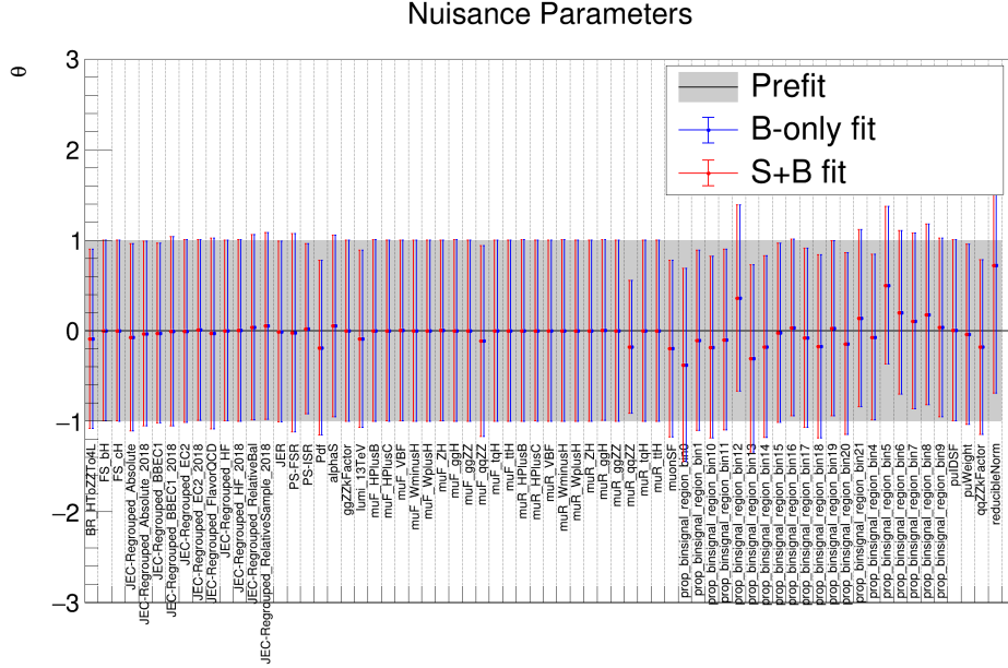
Figure 4.18: The best-fit values of the nuisance parameters that describe the uncertainty model of the background estimation in the baseline scenario. These values are determined in a fit to data in the sideband region of the Higgs boson candidate mass.
