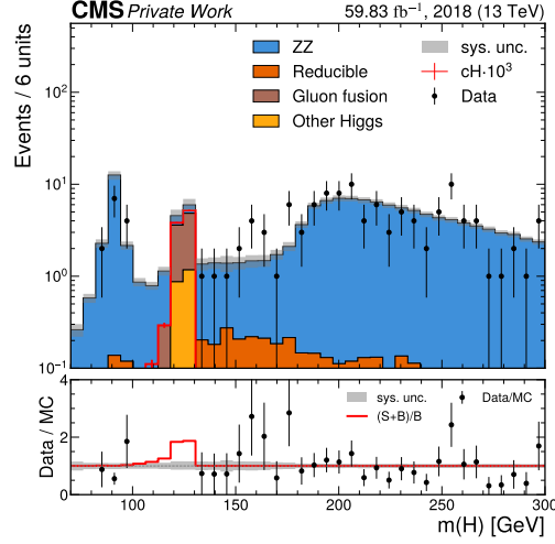
Figure 4.13: The mass spectrum of the Higgs boson candidate, showing the agreement between the 2018 dataset and simulation in the sideband regions of the spectrum. The contribution from a cH(ZZ \rightarrow 4\mu)_{\kappa_C} signal, scaled by a factor 10^3 for better visibility, is also shown. The signal contribution is clearly concentrated around the Higgs boson mass of m(H) = 125 GeV, as expected.
