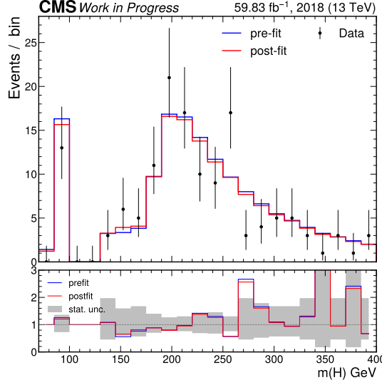
Figure 4.17: The pre- and post-fit distributions of the background estimation model in the sideband region of the Higgs boson candidate mass spectrum for the 2018 data taking era of the CMS detector. The distribution observed for data is also shown and, in the lower panel, the ratio of the pre-fit and post-fit distributions with respect to data can be seen. A reasonable agreement to data is observed already for the pre-fit distribution, indicating that the model is able to describe the data well within the statistical fluctuations observed in data.
