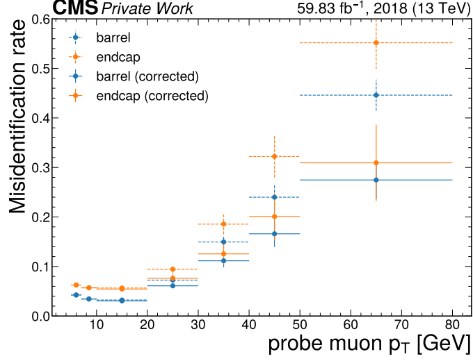
Figure 4.12: The muon misidentification rate in bins of the probe muon transverse momentum, in both the barrel and endcap regions. The dotted lines represent the uncorrected misidentification rate while the solid lines represent the misidentification rate where contributions from WZ \rightarrow 3\ell\nu processes are subtracted.
