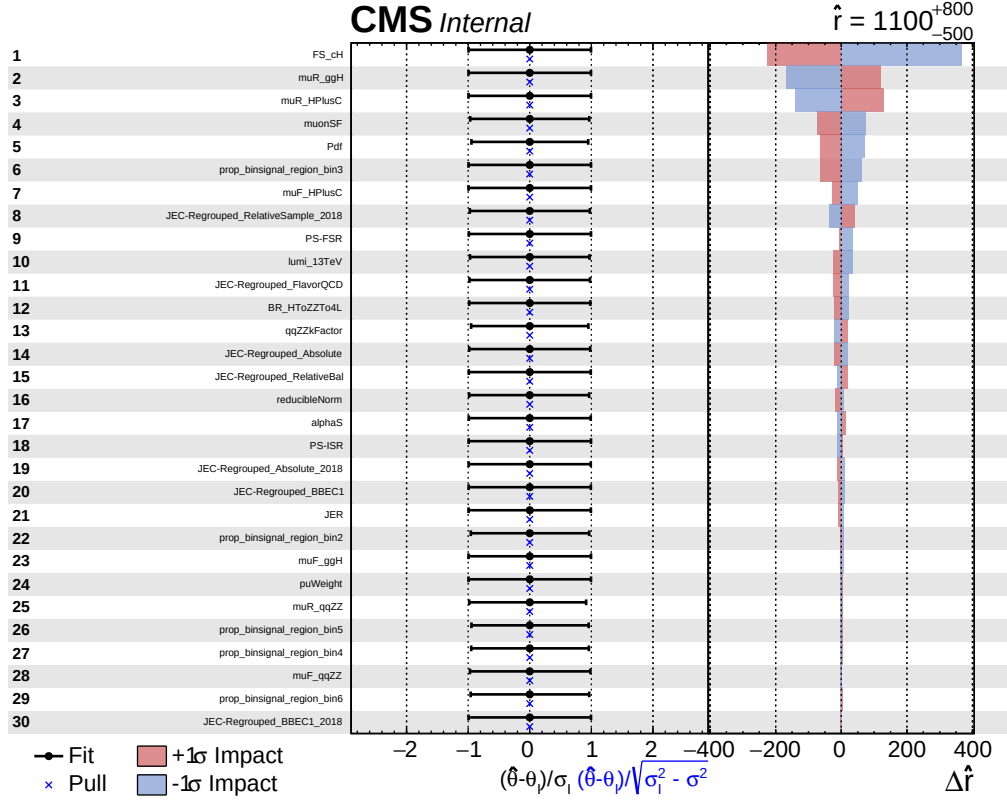
Figure 4.16: Figure showing the 30 leading uncertainty sources in a fit of the \sigma\mathcal{B}(\text{cH}(\text{ZZ} \rightarrow 4\mu))_{\kappa_c} signal strength, ordered by their relative impact on the fit. In the left panel the nuisance parameter names are shown. In the central panel, the fitted nuisance parameter values as well as their so-called pulls are shown. On the right, the \Delta\hat{r}_i values are shown for the \pm\sigma variations associated with each nuisance parameter.
