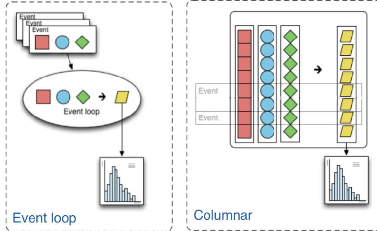
Figure 4: A representation of event loop based and columnar based analysis approaches can be seen on the left and right respectively [97]. The squares, circles and diamonds represent event data that is transformed via an algorithm into output that is histogrammed, represented by the trapezoids.
