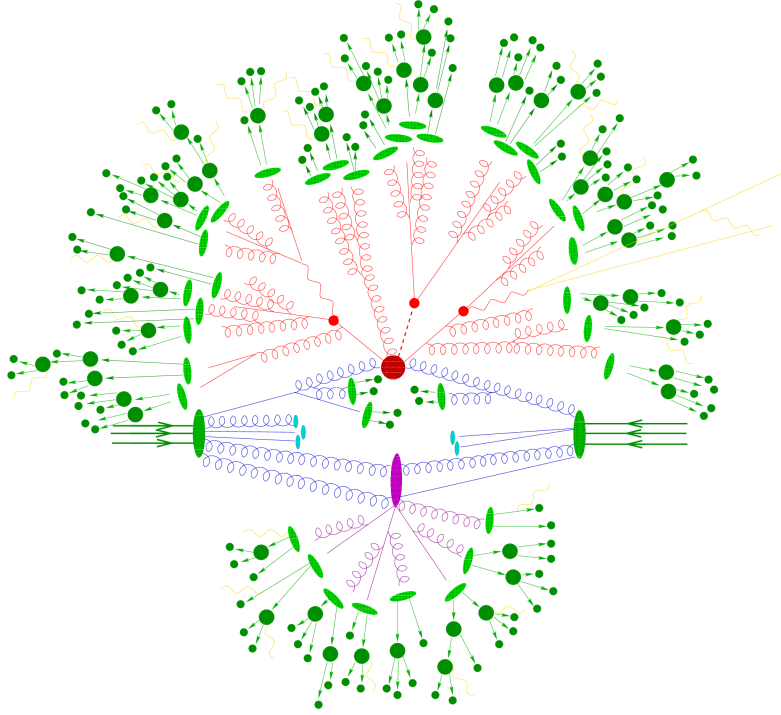
Figure 3.15: An overview of what an event simulation may look like [80]. The initial state particles originating from the protons are shown in blue. The hard scattering process is represented in red. Additional, soft scatterings are represented in purple. The hadronisation to form colourless hadrons (represented by dark green circles) is represented by the light green ellipses. Additional photon radiation is represented in yellow.
