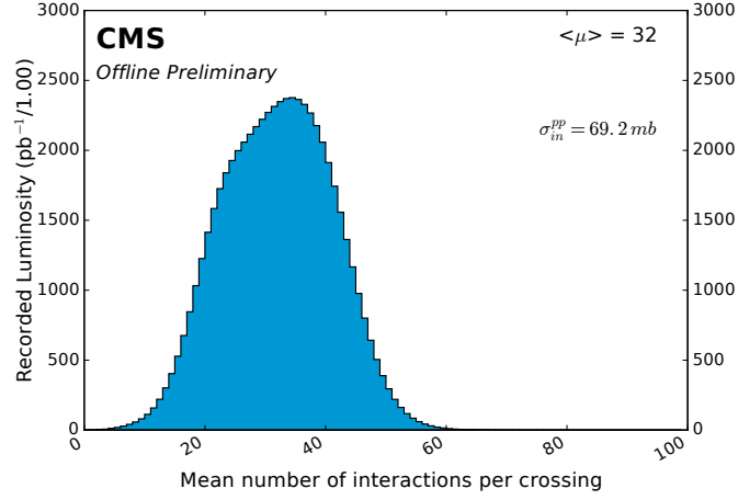
Figure 3.14: The distribution of the mean number of pileup interactions per bunch crossing, measured for the 2018 era of the Run-2 dataset of the CMS detector [79].
