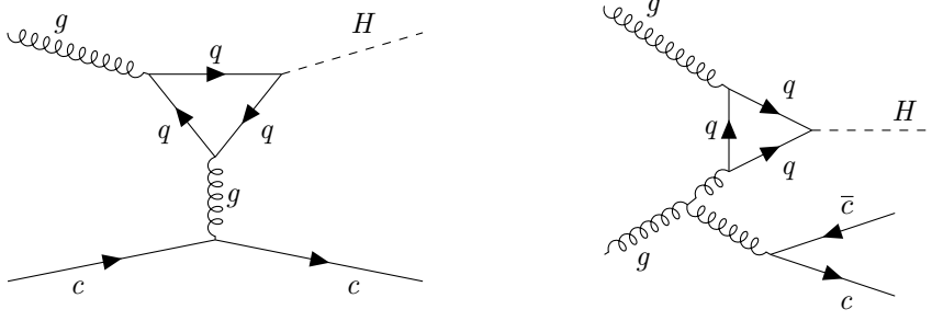
Figure 4.11: Feynman diagrams that represent how contributions to the gluon fusion process may produce cH final states that are insensitive towards \kappa_c . The left diagram shows an example of an explicit higher order perturbative QCD correction to the gluon fusion process that produces a cH final state. The right diagram shows an example where a cH final state is produced due to gluon radiation and subsequent gluon splitting g \rightarrow c\bar{c} , which may be described via parton showering.
