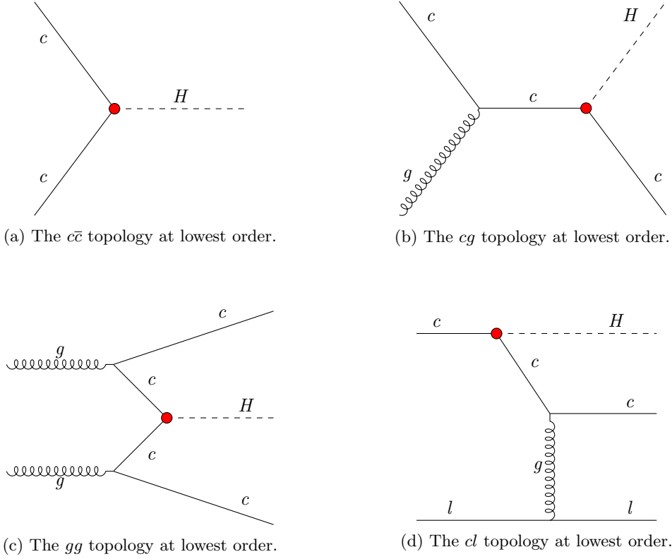
Figure 4.5: Examples of feynman diagrams that illustrate the four different event topologies generated in the cH(ZZ \rightarrow 4\mu) sample at the lowest order. The red dots represent the y_c coupling.
