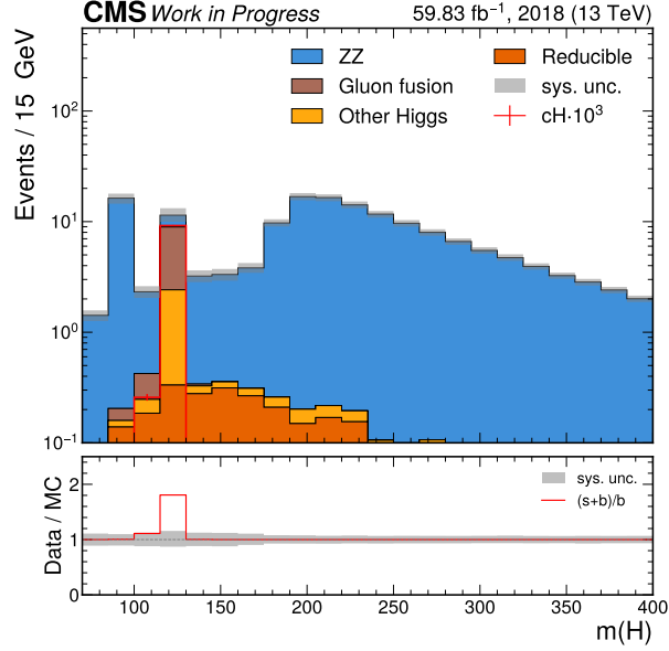
Figure 4.10: The mass spectrum of the Higgs boson candidate, showing the agreement between the 2018 dataset and simulation in the side band regions of the spectrum. The contribution from a cH(ZZ \rightarrow 4\mu) signal, scaled by a factor 10^3 for better visibility, is also shown. The signal contribution is clearly concentrated around the Higgs boson mass of m(H) = 125 GeV, as expected.
