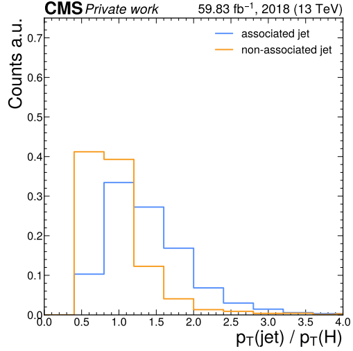
(b) The p_T(\text{jet})/p_T(H) template.
