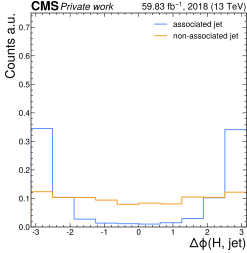
(a) The \Delta\phi(H, \text{jet}) template.
