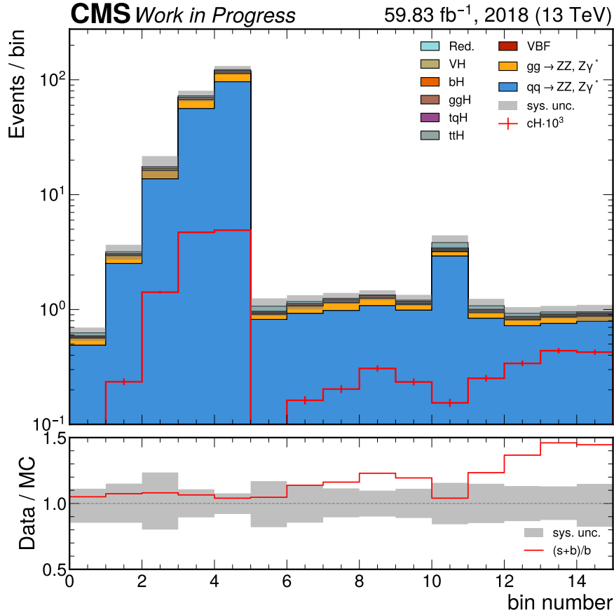
Figure 3.12: The unrolled discriminator distribution representing the CvsB discriminator in three bins of the CvsL discriminator for the selected jet of the reconstructed \text{cH}(\text{ZZ} \rightarrow 4\mu) candidates. As can be seen in the lower panel, the relative contribution of a \text{cH}(\text{ZZ} \rightarrow 4\mu) signal in each bin generally increases with increasing bin number. The region most enriched with signal are the last bins on the right side of the distributions, which as expected, corresponds to selected jets with both a high CvsL and CvsB value. The \text{cH}(\text{ZZ} \rightarrow 4\mu) signal contribution is scaled by a factor of 10^3 to improve its visibility.
