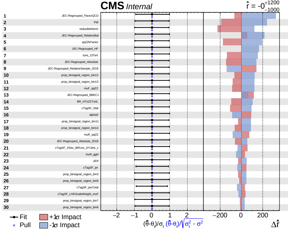
Figure 3.13: Figure showing the 30 leading uncertainty sources in a fit of \sigma \text{BR}(CH(ZZ \rightarrow 4\mu)) , ordered by their relative impact on the fit. In the left panel the nuisance parameter names can be seen. In the central panel, the fitted nuisance parameter values as well as their so-called pulls are shown. On the right, the \Delta \hat{r}_i values can be seen for the \pm\sigma variations associated with each nuisance parameter.
