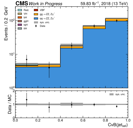
(f) CvsB discriminator of the selected jet.
