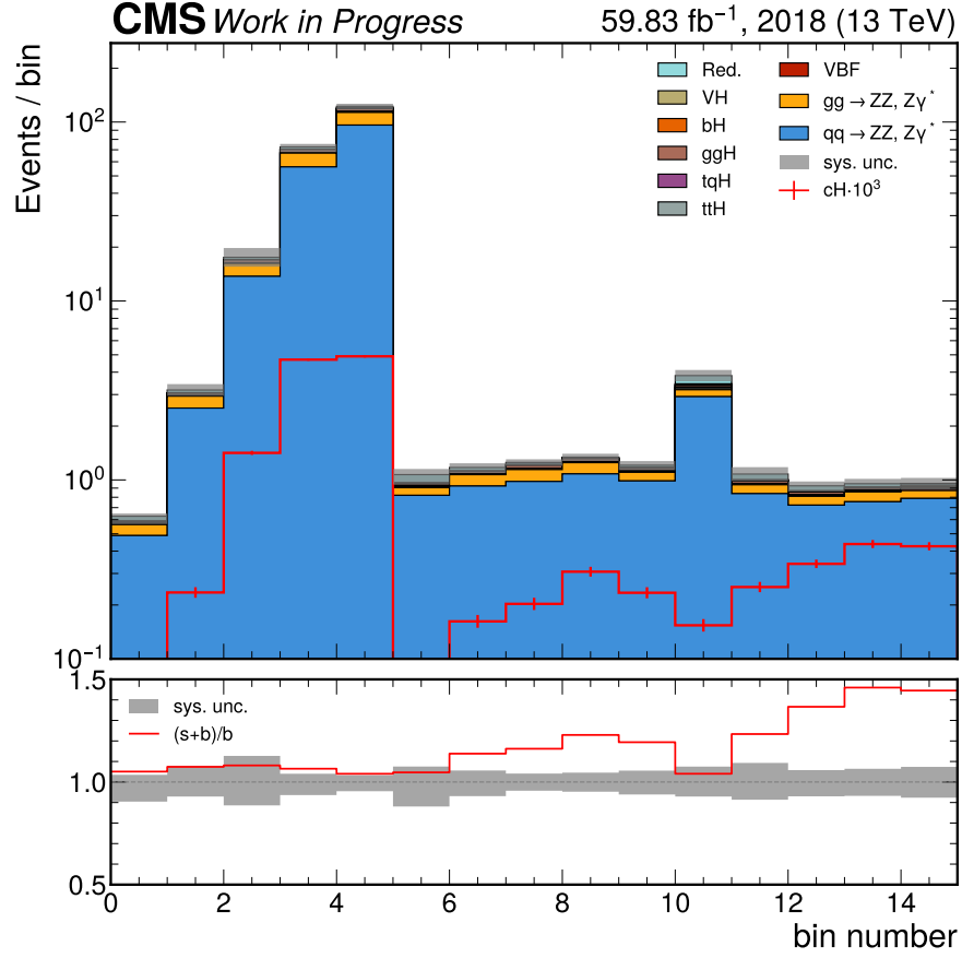
Figure 3.9: The unrolled discriminator distribution representing the CvsB discriminator in three bins of the CvsL discriminator for the selected jet of the reconstructed cH(ZZ \rightarrow 4\mu) candidates. As can be seen in the lower panel, the relative contribution of a cH(ZZ \rightarrow 4\mu) signal in each bin generally increases with increasing bin number. The region most enriched with signal are the last bins on the right side of the distributions, which as expected, corresponds to selected jets with both a high CvsL and CvsB value.
