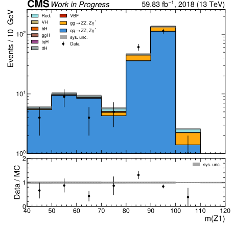
(b) Mass of the Z_1 candidate.
