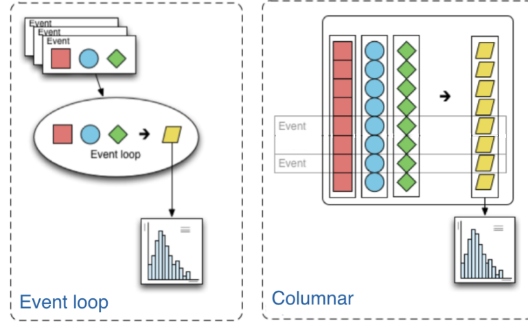
Figure 1: A representation of event loop based and columnar based analysis approaches can be seen on the left and right respectively [73]. The squares, circles and diamonds represent event data that is transformed via an algorithm into output that is histogrammed, represented by the trapezoids.
