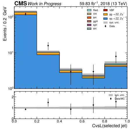
(e) CvsL discriminator of the selected jet.
