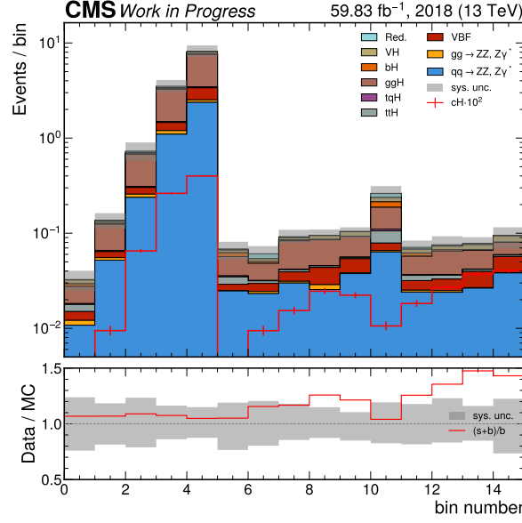
(a) Higgs boson candidate mass limited to [100 GeV, 130 GeV].
