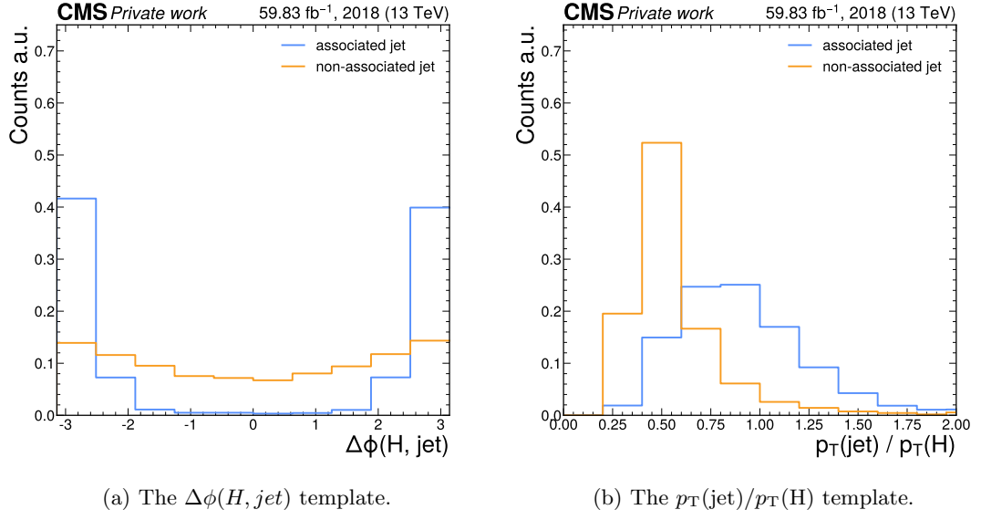
Figure 4: The \Delta\phi(H, jet) and p_T(jet)/p_T(H) templates in the 30-50 GeV bin of the Higgs candidate mass.
