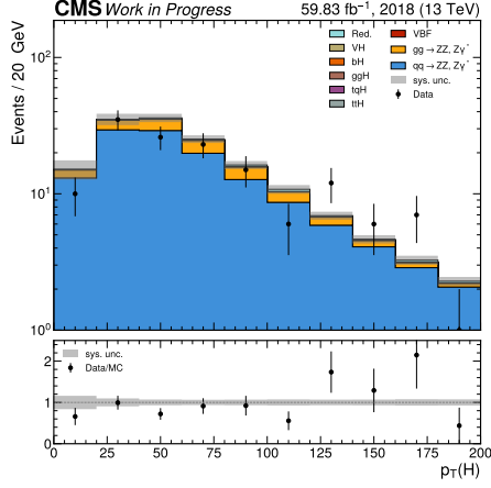
(a) Higgs boson candidate transverse momentum.
