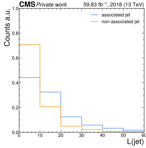
Figure 3.2: The distribution of the jet selection likelihood \mathcal{L}(\text{jet}) in simulated \text{cH}(\text{ZZ} \rightarrow 4\mu) events, shown for associated and non-associated jets in which an associated jet can be identified via a parton-to-jet matching. It can be seen that on average, applying the jet selection algorithm on the associated jet produces a higher likelihood value than on non-associated jets, as expected.
