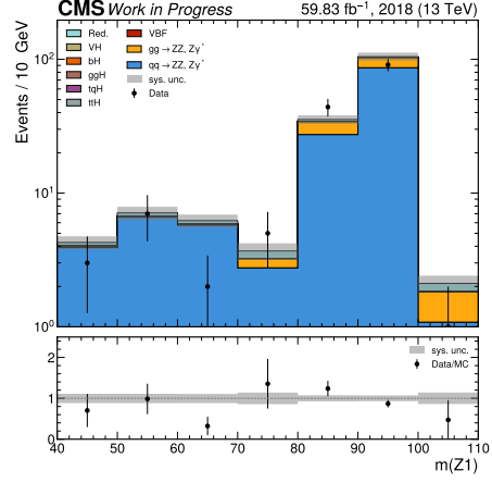
(b) Mass of the Z_1 candidate.
