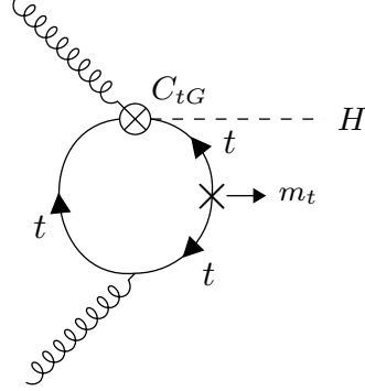
Figure 1.6: A modification of the gluon fusion process with a top quark loop by including the vertex introduced by the top quark CMD operator. Note that the arrows indicate chirality and not momentum flow. A chirality flip, denoted by the cross, proportional to the top quark mass m_t is required for the inclusion of the top quark CMD vertex.
