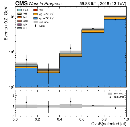
(f) CvsB discriminator of the selected jet.
