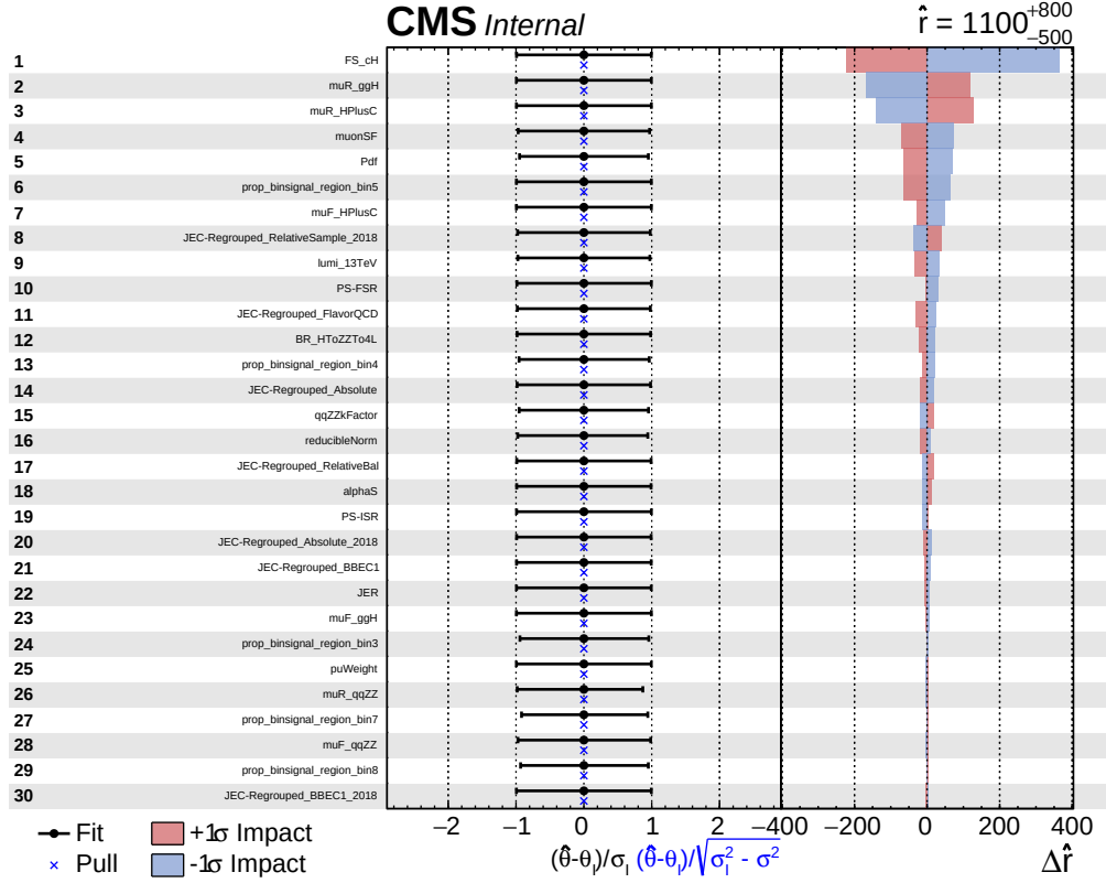
Figure 3.14: Figure showing the 30 leading uncertainty sources in a fit of \sigma \text{BR}(CH(ZZ \rightarrow 4\mu)) , ordered by their relative impact on the fit. In the left panel the nuisance parameter names can be seen. In the central panel, the fitted nuisance parameter values as well as their so-called pulls are shown. On the right, the \Delta \hat{r}_i values can be seen for the \pm\sigma variations associated with each nuisance parameter.
