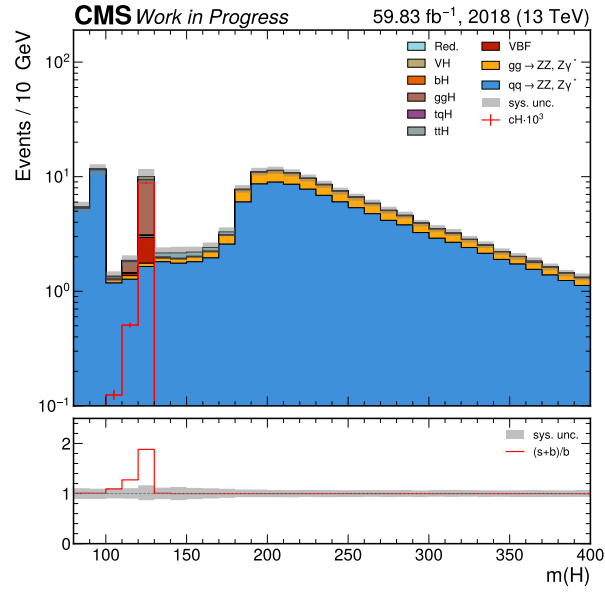
Figure 3.12: The Higgs boson candidate mass spectrum, used as a discriminator to derive expected 95% CL CL_s upper limits on \sigma BR(cH(ZZ \rightarrow 4\mu)) in the baseline scenario. The region around the Higgs boson mass peak at m(H) = 125 GeV is clearly enriched in signal, which is scaled by a factor of 10^3 here to improve visibility.
