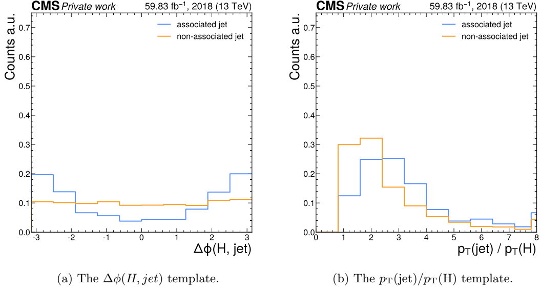
Figure 2: The \Delta\phi(H, jet) and p_T(jet)/p_T(H) templates in the 0-15 GeV bin of the Higgs candidate mass.
