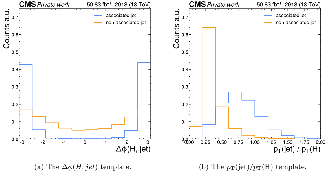
Figure 5: The \Delta\phi(H, jet) and p_T(jet)/p_T(H) templates in the 50-100 GeV bin of the Higgs candidate mass.
