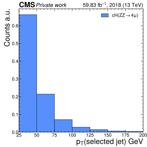
Figure 3.3: The distribution of the selected jet's transverse momentum in simulated \text{cH}(\text{ZZ} \rightarrow 4\mu) events. As expected, the majority of jets come at relatively low transverse momenta.
