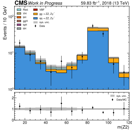
(c) Mass of the Z_2 candidate.
