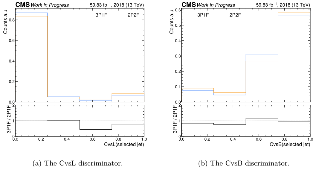
Figure 8: A comparison between the 2P2F and 3P1F regions of the reducible background estimation, looking specifically at the shape of the DeepJet c-tagging discriminator distributions. A reasonable agreement is observed, with the most significant differences being observed in more sparsely populated bins.
