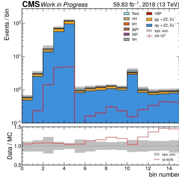
(b) Inclusive Higgs boson candidate selection.
