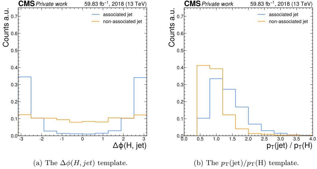
Figure 3: The \Delta\phi(H, jet) and p_T(jet)/p_T(H) templates in the 15-30 GeV bin of the Higgs candidate mass.
