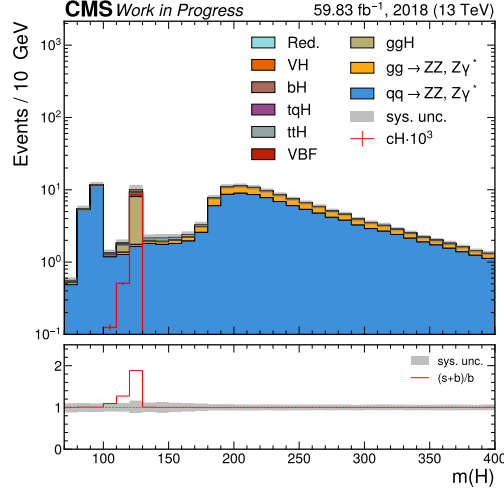
Figure 3.12: The Higgs boson candidate mass spectrum, used as a discriminator to derive expected upper limits on \sigma\text{BR}(cH(ZZ \rightarrow 4\mu)) in the baseline scenario. The region around the Higgs boson mass peak at m(H) = 125 GeV is clearly enriched in signal, which is scaled by a factor of 10^3 here to improve visibility.
