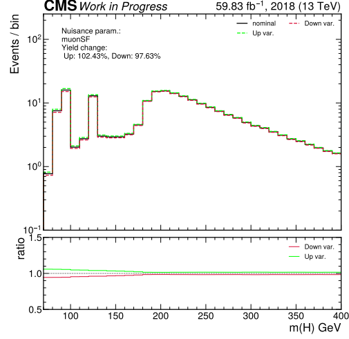
Figure 12: The uncertainty associated with the calibration of muons.
