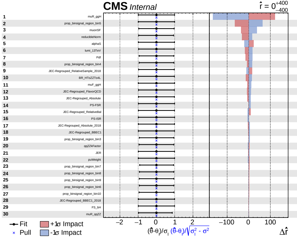
Figure 13: The 30 leading uncertainty sources in a fit of \sigma\mathcal{B}(\text{ch}(\text{ZZ} \rightarrow 4\mu)) with r = 0 , ordered by their relative impact on the fit.
