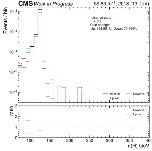
(k) \chi H(ZZ \rightarrow 4\mu) flavour scheme
