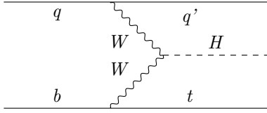
(e) The tqH process.
