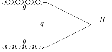
(a) The ggH process.
