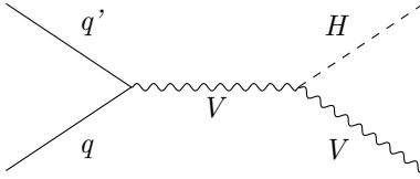
(c) The VH process.
