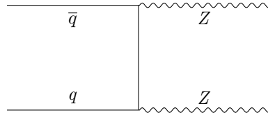
(g) The qq \rightarrow ZZ process.
