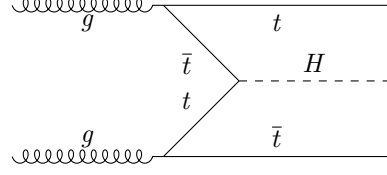
(b) The t\bar{t}H process.
