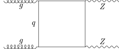
(f) The gg \rightarrow ZZ process.
