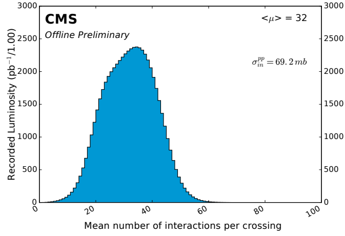
Figure 3.14: The distribution of the mean number of pileup interactions per bunch crossing, measured for the 2018 era of the Run-2 dataset of the CMS detector [75].
