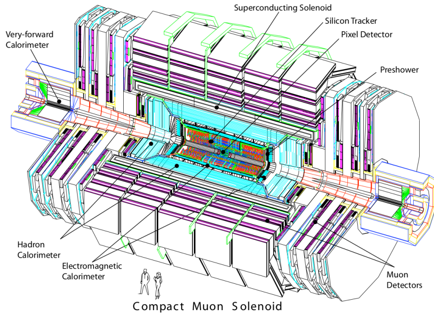
Figure 3.2: An overview of the CMS detector [38], showing the individual subsystems it is composed of.
