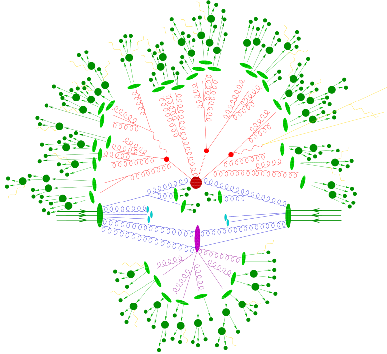
Figure 3.15: An overview of what an event simulation may look like [76]. The initial state particles originating from the protons are shown in blue. The hard scattering process is represented in red. Additional, soft scatterings are represented in purple. The hadronisation to form colourless hadrons (represented by dark green circles) is represented by the light green ellipses. Additional photon radiation is represented in yellow.
