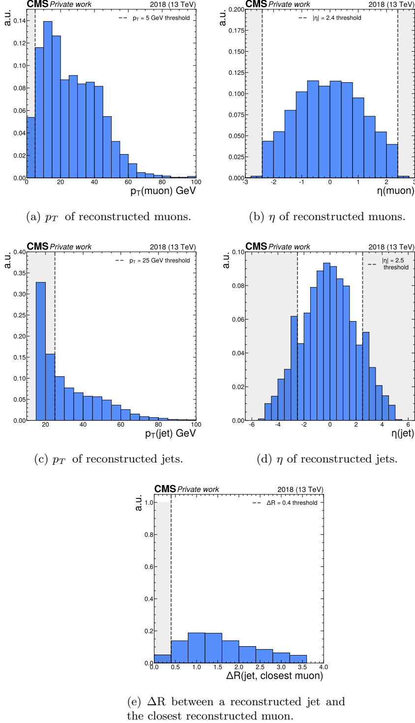
Figure 4.1: Distributions of jet and muon quantities (inclusive in the number of jets and muons) to which selection criteria are applied during the initial muon and jet selection, shown for four-muon events in a simulation of the CH(ZZ \rightarrow 4\mu)_{\kappa_c} process. The thresholds associated with the selection criteria are marked by dashed lines and the region where contributions are removed are shaded.
