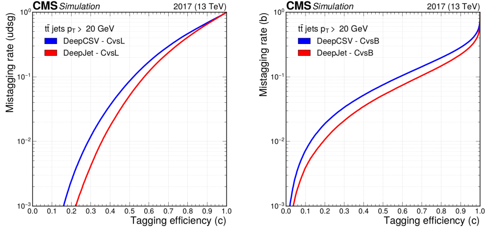
Figure 2.11: Performance of DeepJet algorithm in identifying c jets against b jets and light jets in simulated samples of top quark pair production, in which both top quarks decay hadronically [53]. The x-axis represents the efficiency with which c jets are identified, while the y-axis represents misidentification rate with respect to either b jets or light jets.
