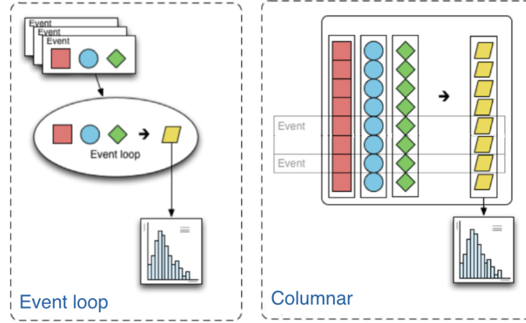
Figure 1: A representation of event loop based and columnar based analysis approaches can be seen on the left and right respectively [68]. The squares, circles and diamonds represent event data that is transformed via an algorithm into output that is histogrammed, represented by the trapezoids.
