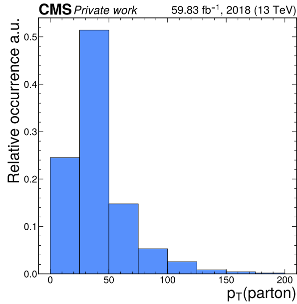
Figure 1.3: Transverse momentum of the parton produced alongside a Higgs boson in a Madgraph5_aMC@NLO [16] simulation of the cH process within the CMS detector, which typically takes on relatively small values.
