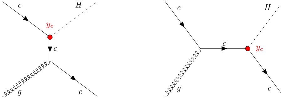
Figure 1.2: The leading-order cH processes through which y_c may be probed as each diagram contains a vertex with a charm quark and Higgs boson, here denoted in red. The corresponding diagrams with an anti-charm quark \bar{c} are implied.
