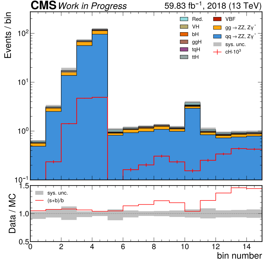
Figure 3.12: The unrolled discriminator distribution representing the CvsB discriminator in three bins of the CvsL discriminator for the selected jet of the reconstructed CH(ZZ \rightarrow 4\mu) candidates. As can be seen in the lower panel, the relative contribution of a CH(ZZ \rightarrow 4\mu) signal in each bin generally increases with increasing bin number. The region most enriched with signal are the last bins on the right side of the distributions, which as expected, corresponds to selected jets with both a high CvsL and CvsB value. The CH(ZZ \rightarrow 4\mu) signal contribution is scaled by a factor of 10^3 to improve its visibility.
