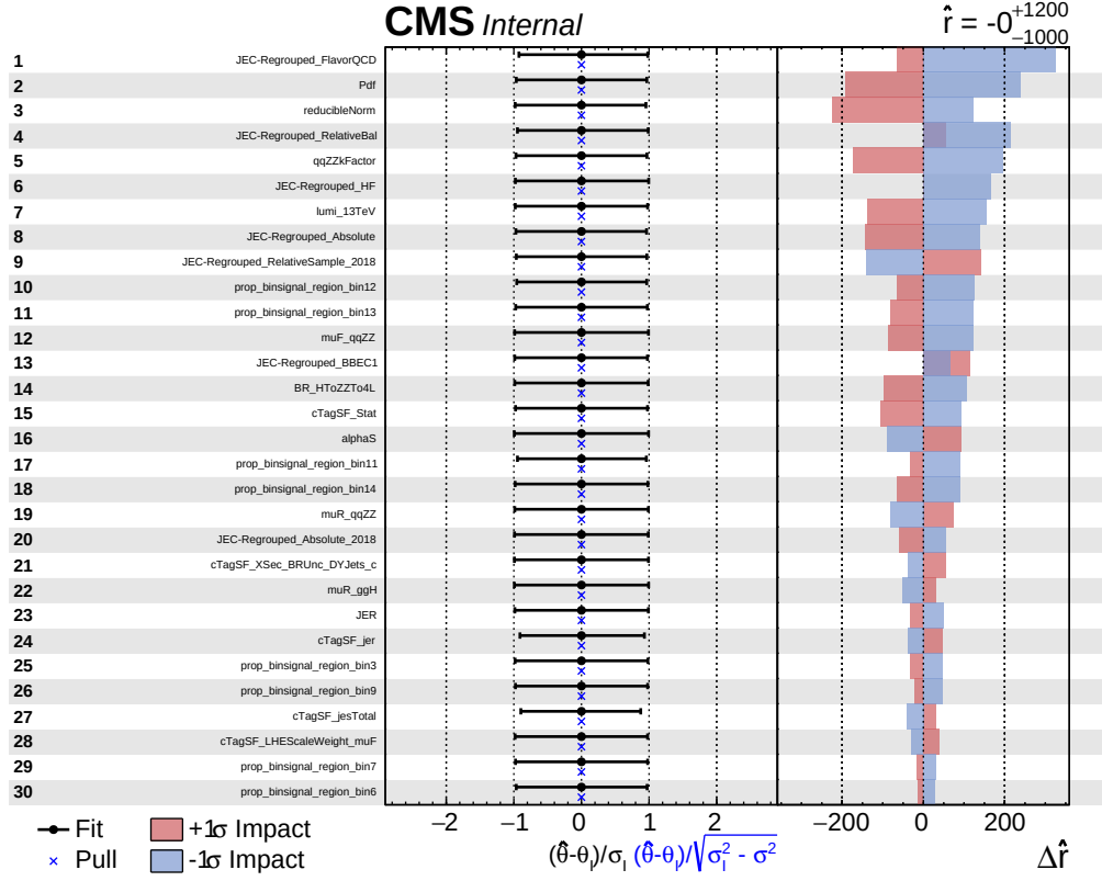
Figure 3.13: Figure showing the 30 leading uncertainty sources in a fit of \sigma\text{BR}(c\text{H}(ZZ \rightarrow 4\mu)) , ordered by their relative impact on the fit. In the left panel the nuisance parameter names can be seen. In the central panel, the fitted nuisance parameter values as well as their so-called pulls are shown. On the right, the \Delta\hat{r}_i values can be seen for the \pm\sigma variations associated with each nuisance parameter.
