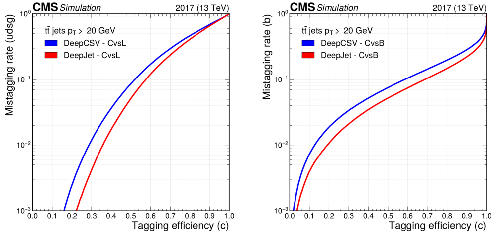
Figure 2.11: Performance of DeepJet algorithm in identifying c jets against b jets and light jets in simulated samples of top quark pair production ( t\bar{t} ), where both top quarks decay hadronically [53]. The x-axis represents the efficiency with which c jets are identified, while the y-axis represents misidentification rate with respect to either b jets or light jets.
