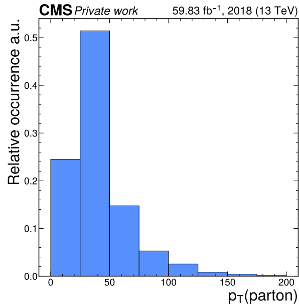
Figure 1.4: Transverse momentum of the parton produced alongside a Higgs boson in a Madgraph5_aMC@NLO [16] simulation of the cH process within the CMS detector, which typically takes on relatively small values.
