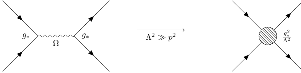
Figure 1.7: Feynman diagrams depicting a resonant process in which the new mediator particle \Omega is created (left) and the approximate description of this in an EFT, where the diagram is reduced to a four-point interaction.
