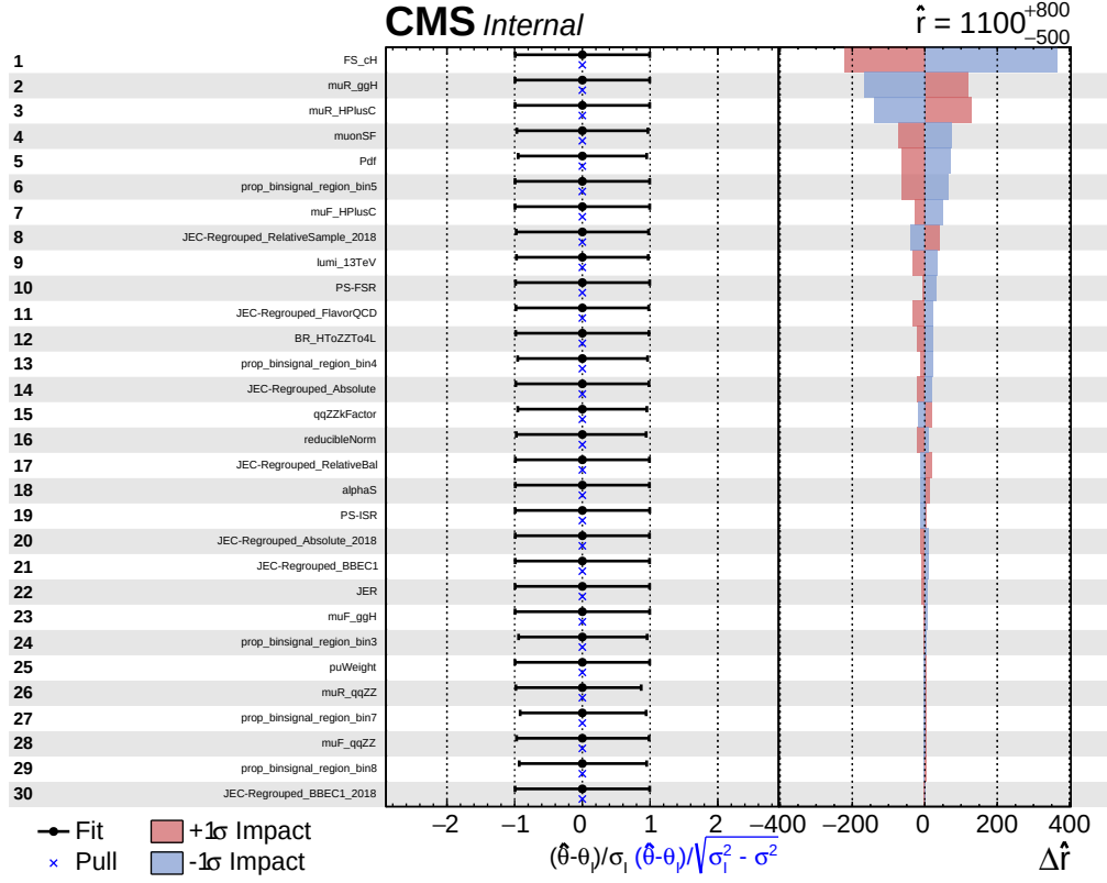
Figure 3.14: Figure showing the 30 leading uncertainty sources in a fit of \sigma\mathcal{B}(\text{ch}(ZZ \rightarrow 4\mu)) , ordered by their relative impact on the fit. In the left panel the nuisance parameter names can be seen. In the central panel, the fitted nuisance parameter values as well as their so-called pulls are shown. On the right, the \Delta\hat{r}_i values can be seen for the \pm\sigma variations associated with each nuisance parameter.
