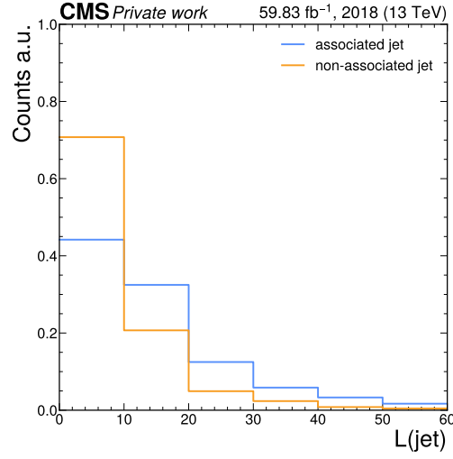
Figure 3.2: The distribution of the jet selection likelihood \mathcal{L}(\text{jet}) , in simulated cH(ZZ \rightarrow 4\mu) events in which an associated jet can be identified via a parton-to-jet matching, for associated and non-associated jets. It can be seen that on average, applying the jet selection algorithm on the associated jet produces a higher likelihood value than on non-associated jets, as expected.
