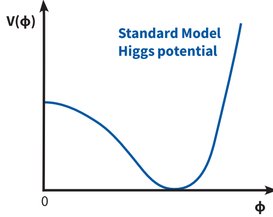
Figure 1.2: A sketch of the shape of the Higgs potential in the Standard Model, which is simplified by showing a cross section of the two dimensional potential. A non-stable maximum at the center of a potential can be seen alongside a stable configuration in a non-zero ground state.
