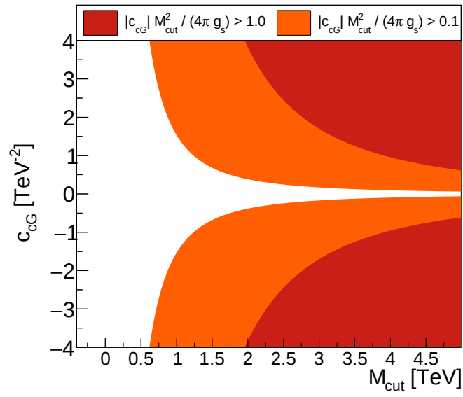
Figure 1.8: Diagram showing the plane spanned by \tilde{C}_{cG} and M_{cut} for the CMD operator [PhenoPaper]. The white region shows the region in which the perturbativity requirement is well satisfied. In the orange region represents the transition region to the red region, in which the perturbativity requirement is no longer valid.
