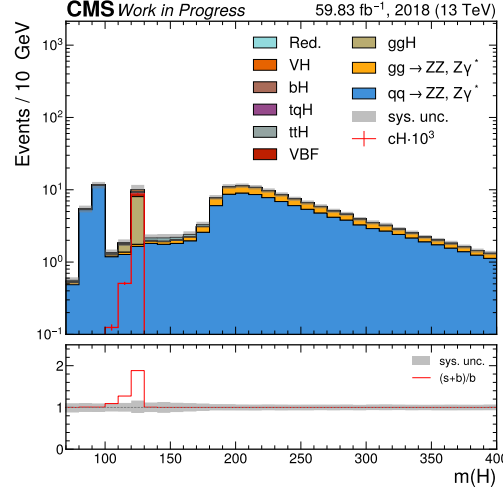
Figure 3.12: The Higgs boson candidate mass spectrum, used as a discriminator to derive expected upper limits on \sigma\text{BR}(\text{cH}(\text{ZZ} \rightarrow 4\mu)) in the baseline scenario. The region around the Higgs boson mass peak at m(\text{H}) = 125 GeV is clearly enriched in signal, which is scaled by a factor of 10^3 here to improve visibility.
