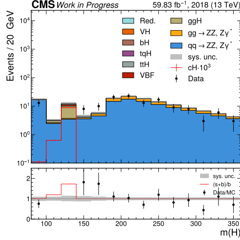
Figure 3.10: The mass spectrum of the Higgs boson candidate, showing the agreement between the 2018 dataset and simulation in the side band regions of the spectrum. The contribution from a cH(ZZ \rightarrow 4\mu) signal, scaled by a factor 10^3 for better visibility, is also shown. The signal contribution is clearly concentrated around the Higgs boson mass of m(H) = 125 GeV, as expected.
