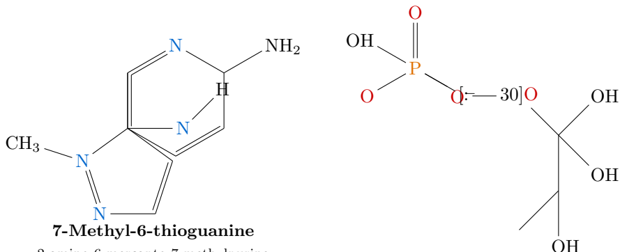
Ribose-1-phosphate
