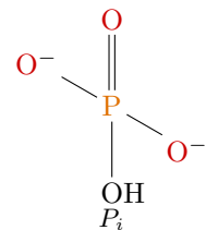
Inorganic phosphate
