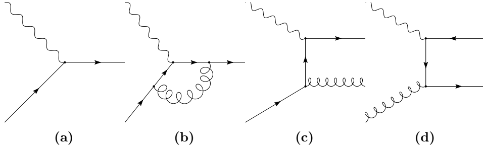
Figure 1.3: Representative LO and NLO DIS Feynman diagrams. While at LO there is a single diagram (a), starting from NLO there are several type of diagrams: virtual corrections (b), radiative corrections (c), and the gluon as initial state parton (d). Note that the list is not exhaustive.
