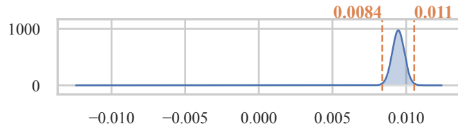
Airfoil Self-Noise
