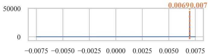
Physiochemical Properties of Protein Tertiary Structure
