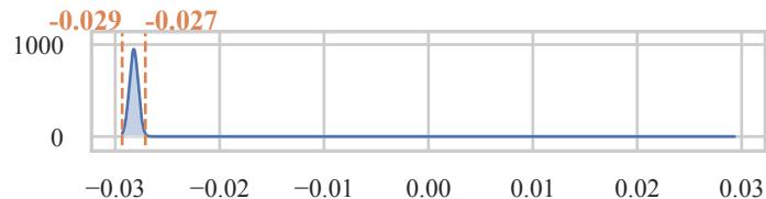
Concrete Strength
