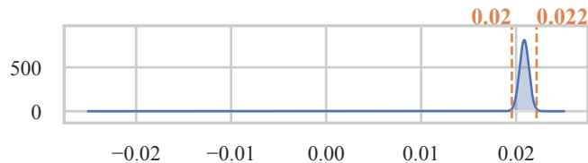
Concrete Strength
