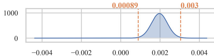
Airfoil Self-Noise
