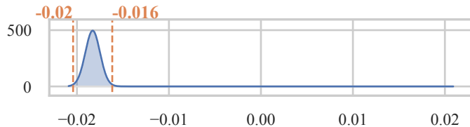
Parkinson's Telemonitoring
