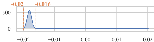
Parkinson's Telemonitoring
