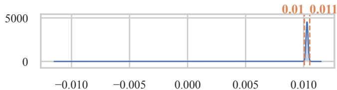
Physiochemical Properties of Protein Tertiary Structure
