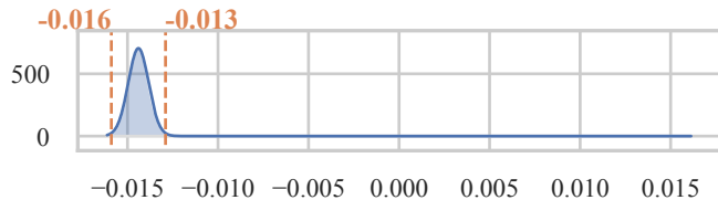
Parkinson's Telemonitoring
