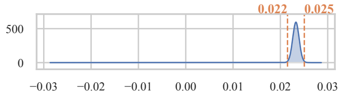
Parkinson's Telemonitoring
