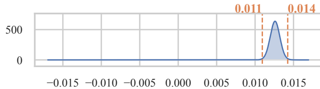
Parkinson's Telemonitoring
