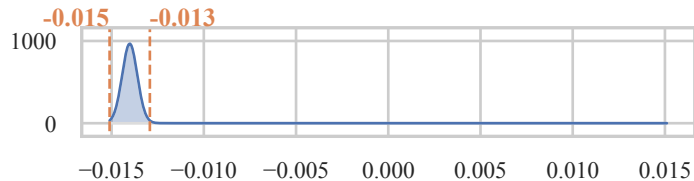
Airfoil Self-Noise
