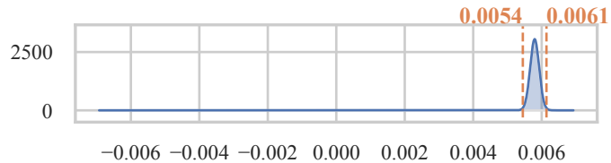
Airfoil Self-Noise
