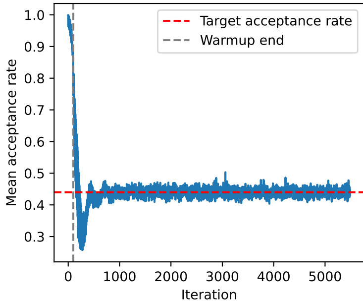
Mean acceptance rate
