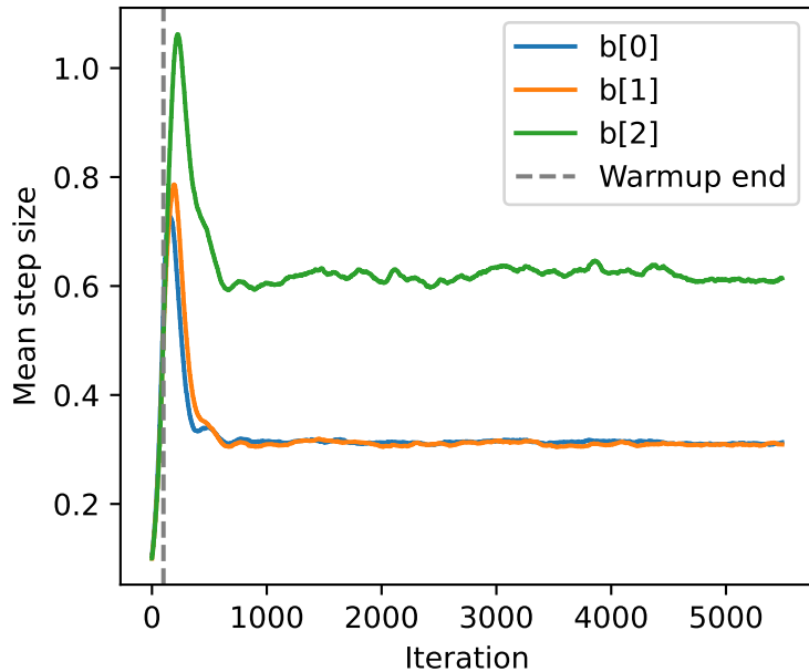
Mean step size (component-wise)
