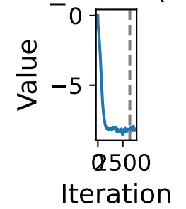
link_coefs.(1, 3)
