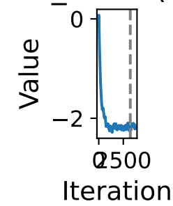
link_coefs.(1, 2)
