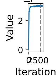
noise_prec.flat
