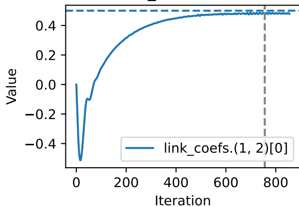
link_coefs.(1, 2)
