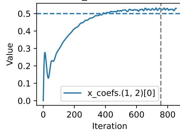
x_coefs.(1, 2)
