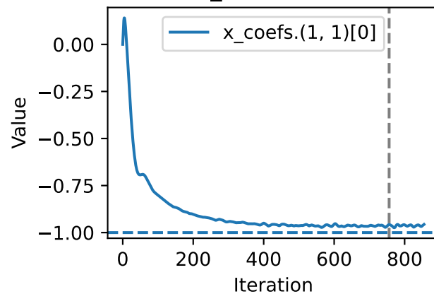
x_coefs.(1, 1)
