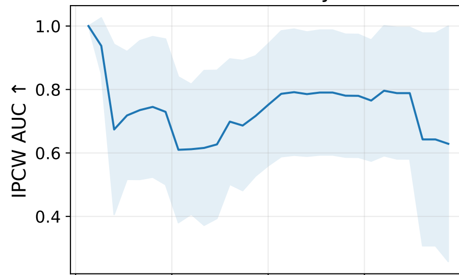
Landmark: 6.3 years
