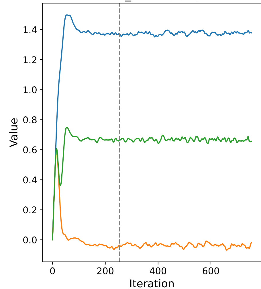
link_coefs.(0, 1)
