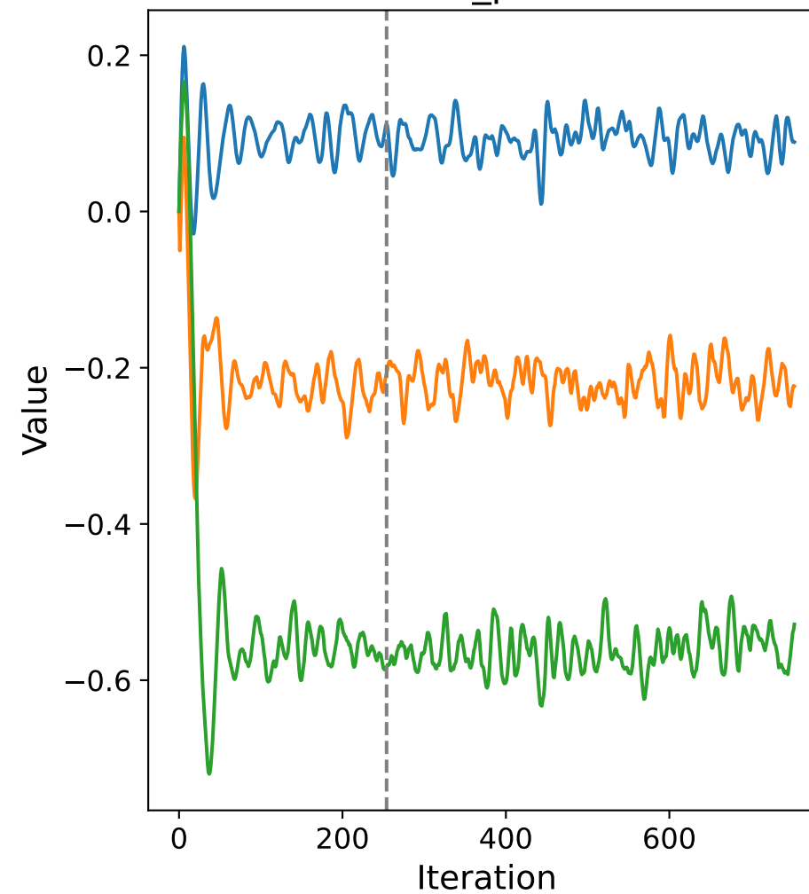
base_hazards.(0, 1).log_k
