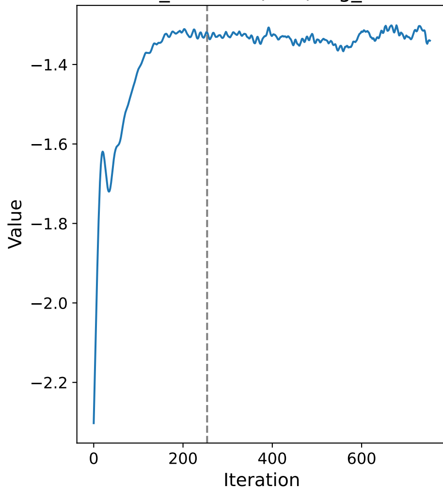
base_hazards.(0, 1).log_lmda
