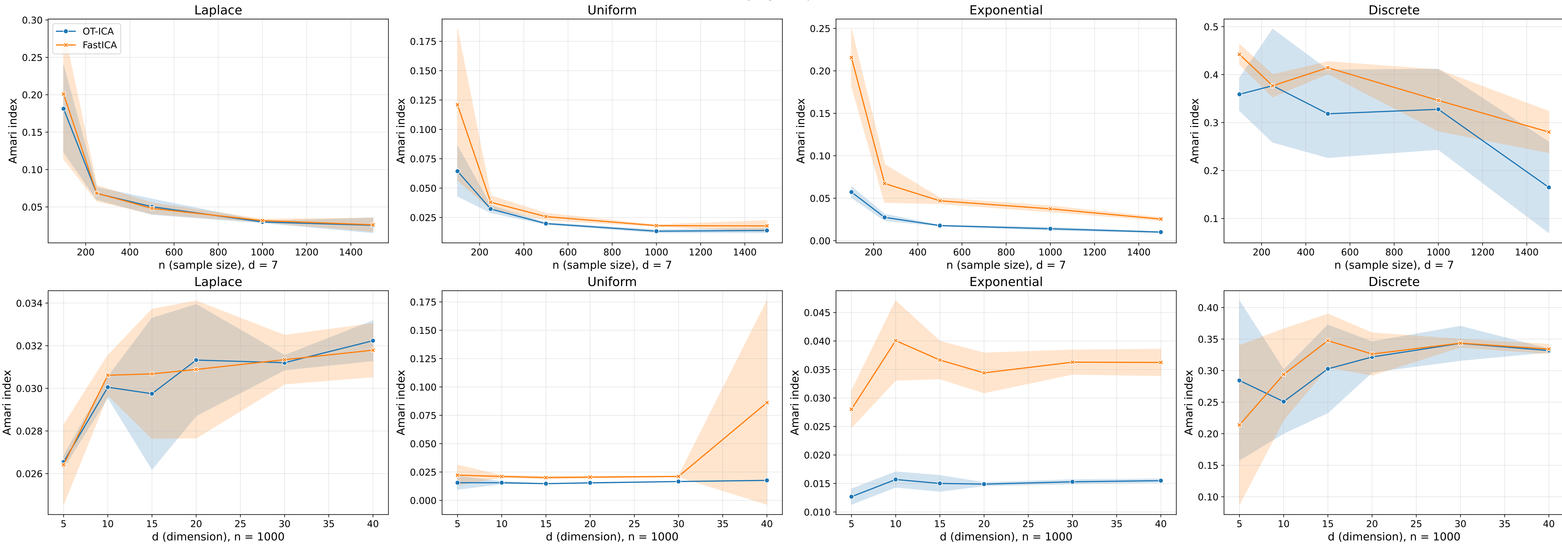
Amari index with varying sample size and dimension
