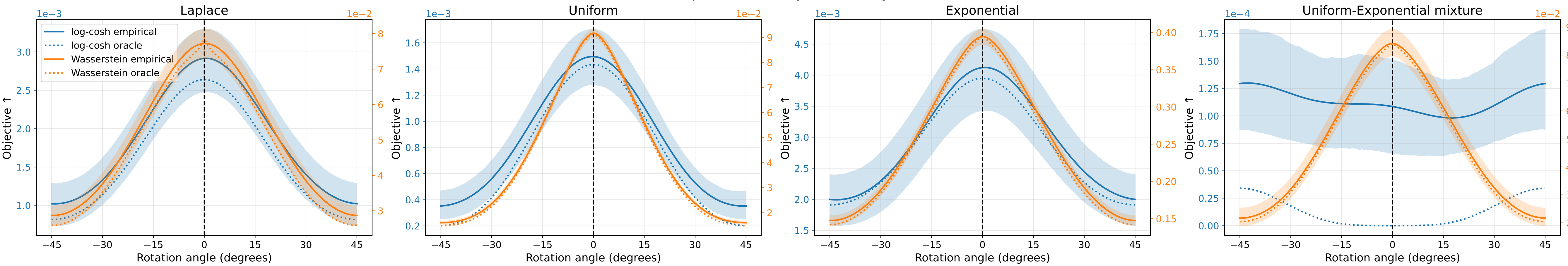
Objective values by rotation angle
