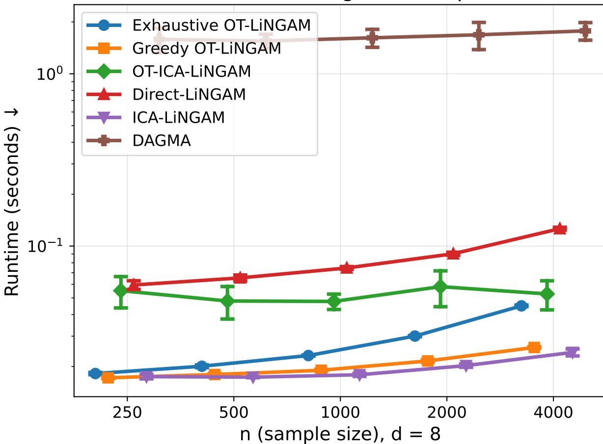
ER2 runtime scaling with sample size
