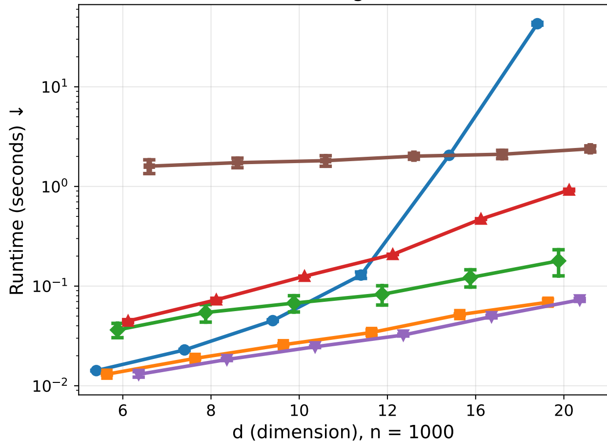
ER2 runtime scaling with dimension
