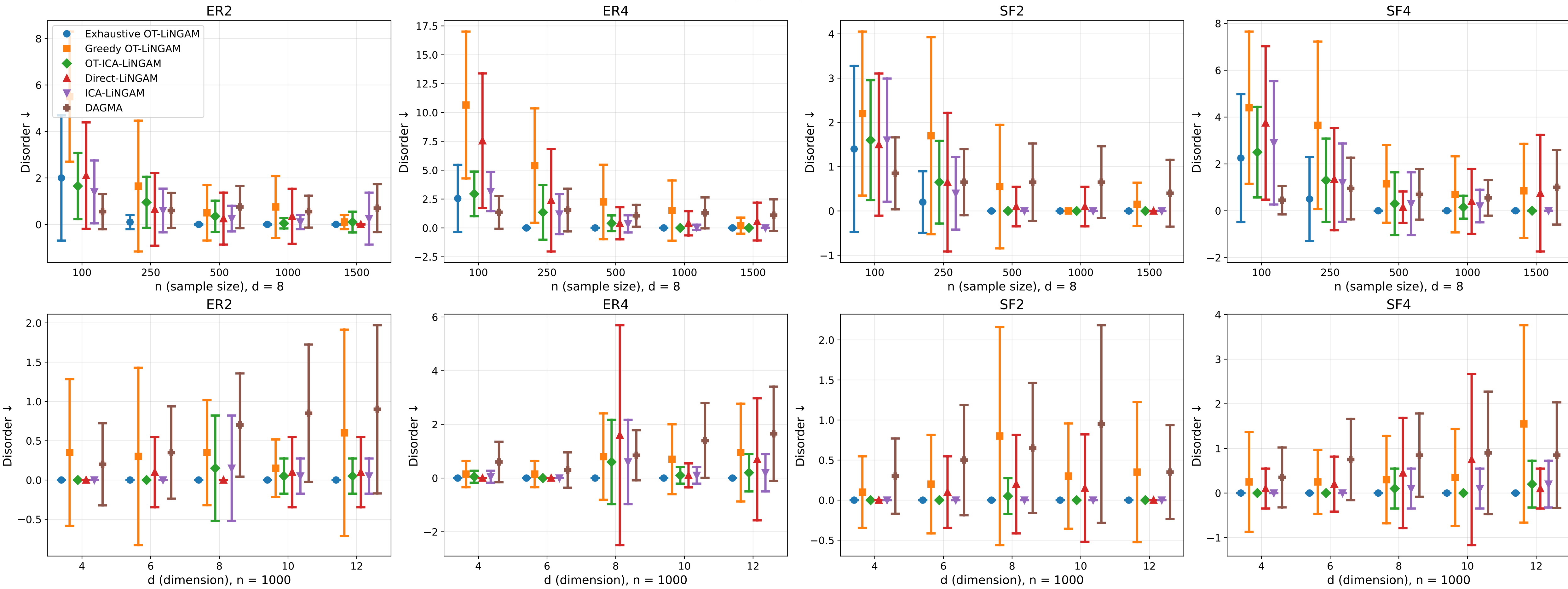
Disorder with varying sample size and dimension
