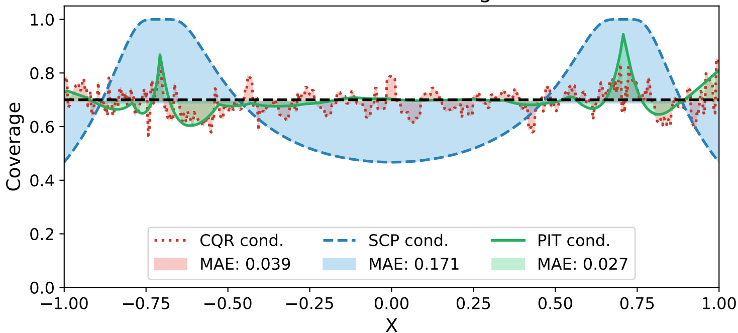
Conditional coverage
