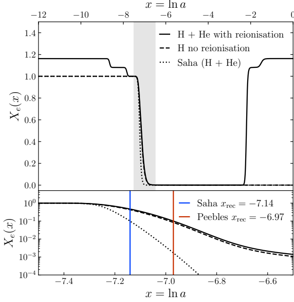
Fig. 9. The free electron fraction X_e as a function of x = \ln a for three configurations: hydrogen and helium with reionisation (solid), hydrogen only without reionisation (dashed), and the pure Saha approximation with both species and without reionisation (dotted), with Y_p = 0.245 where applicable. The bottom panel magnifies the recombination epoch ( -7.5 \leq x \leq -6.5 , shaded grey in the top panel), highlighting the different recombination times.
