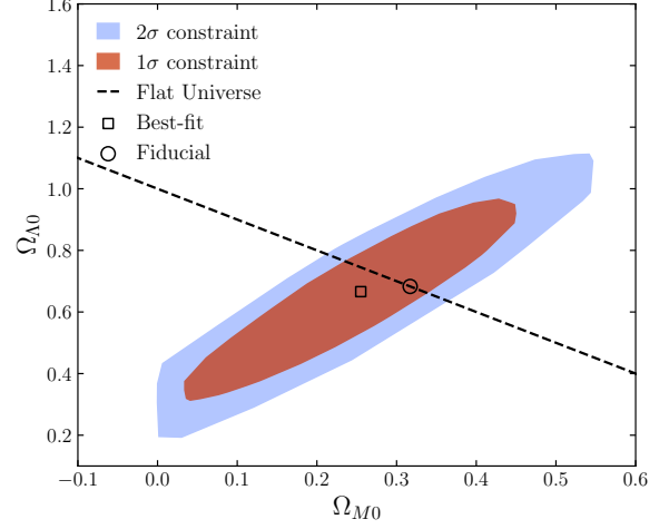
Fig. 6. The regions of sampled points in the (\Omega_{M0}, \Omega_{\Lambda 0}) parameter space within 1\sigma and 2\sigma of the pair associated with the minimal \chi^2 . The diagonal dashed line shows the cosmologies giving a flat Universe; \Omega_{K0} = 1 - \Omega_{M0} - \Omega_{\Lambda 0} = 0 .
