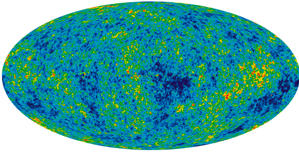
Fig. 1. CMB (NASA WMAP Science Team 2025)
