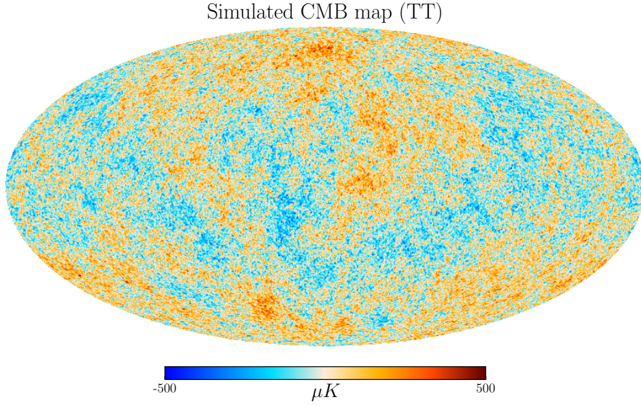
Fig. 21. CMB map produced from the simulated power spectrum. Generated using the Python library healpy (Zonca et al. 2019; Górski et al. 2005).
