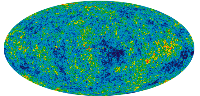
Fig. 1. CMB map (NASA WMAP Science Team 2025).
