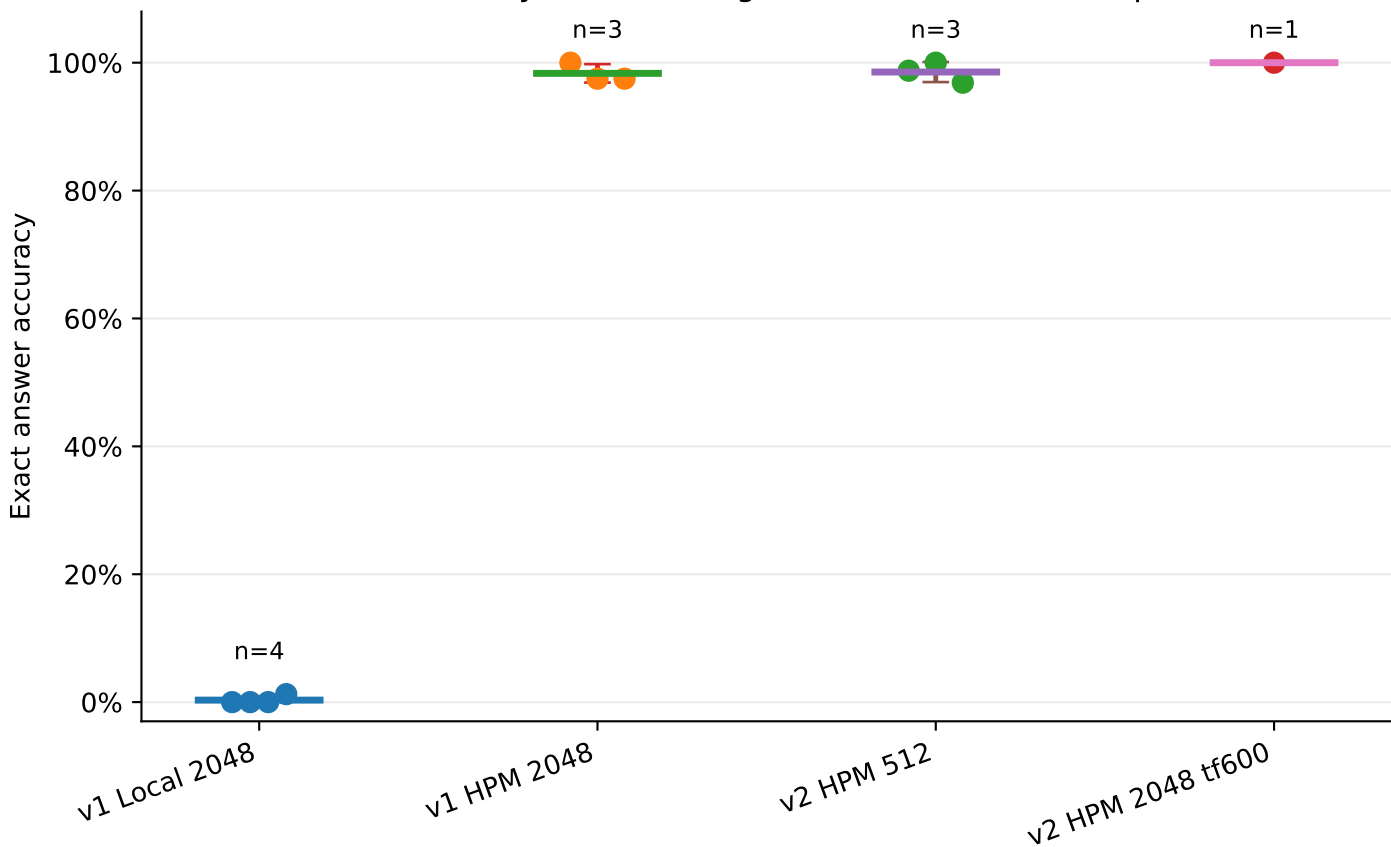
Exact recall by model/configuration with seed-level points
