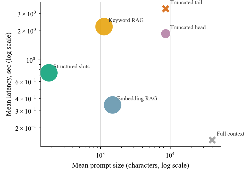
B. Cost/accuracy frontier (marker size = strict-exact accuracy)
