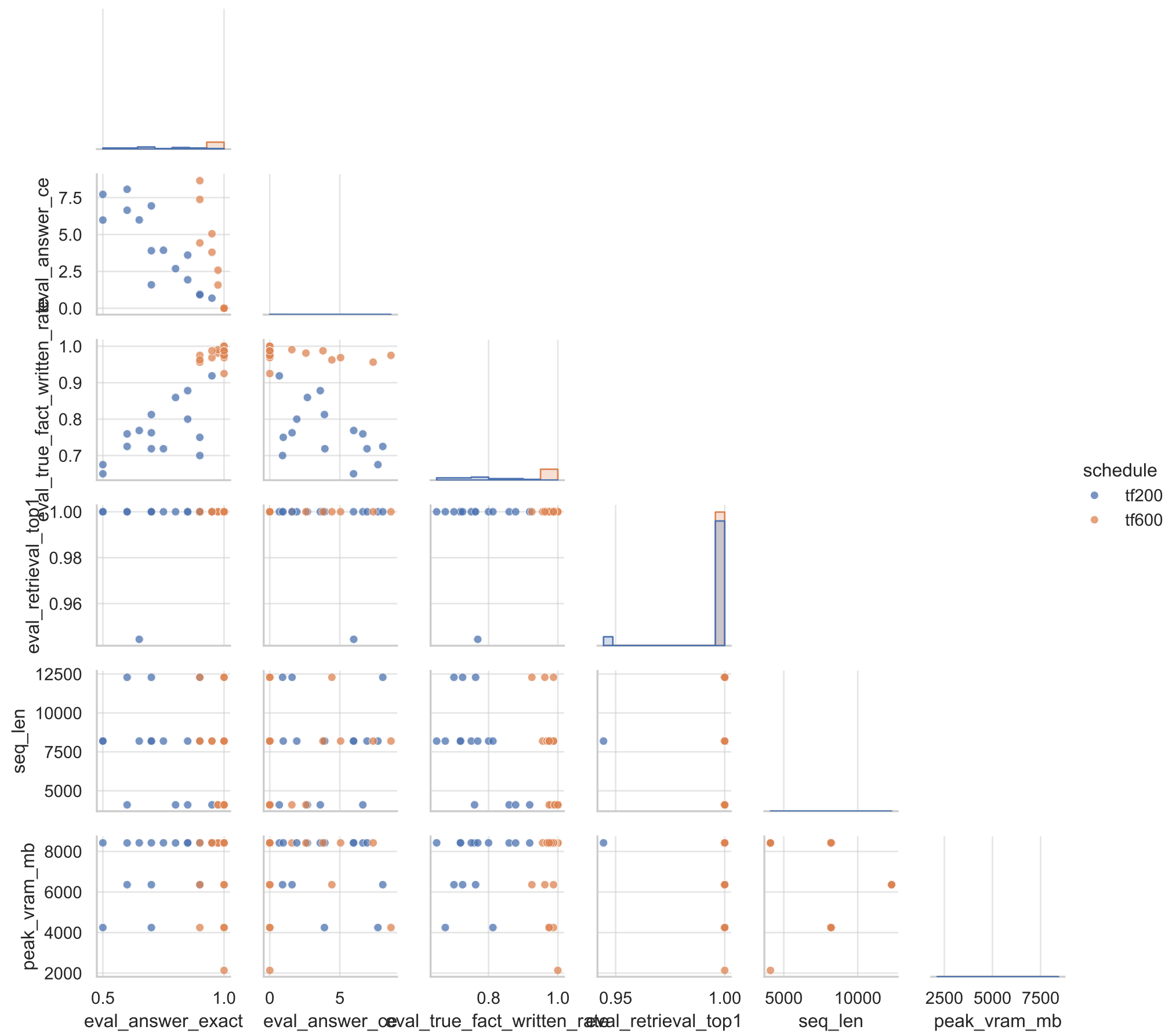
Exploratory PairGrid: aggregate-run relationships
