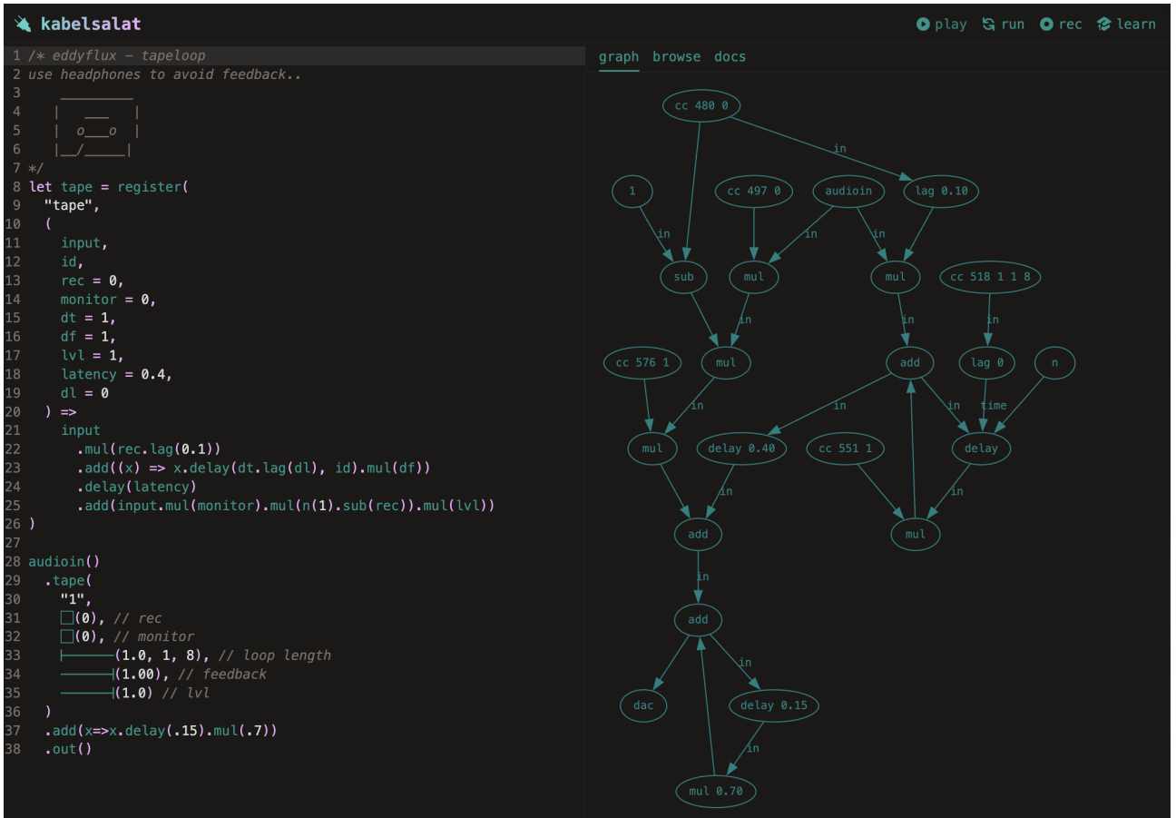
Figure 1: KabelSalat web interface ( https://kabel.salat.dev , accessed on September 27, 2024) running a looper patch. On the left pane pane: source code editor with in-source widgets. On the right pane: the real-time audio graph visualizer.
