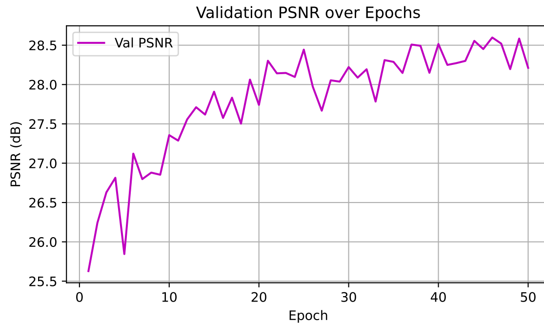
Training with 50 patches/image and validation with 10 patches/image
