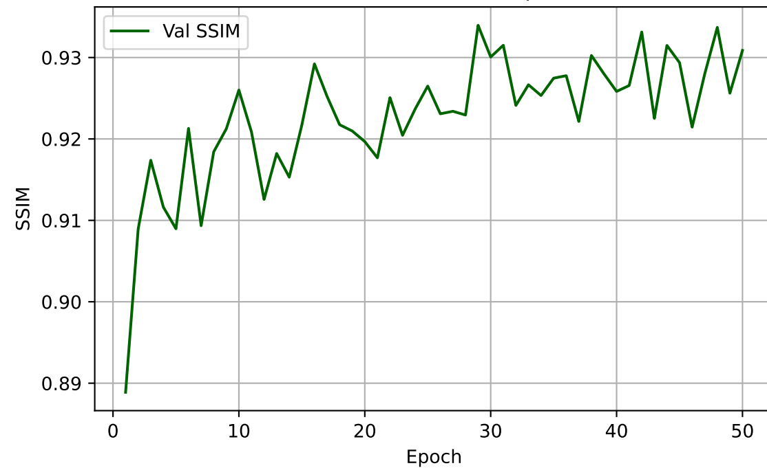
Validation SSIM over Epochs
