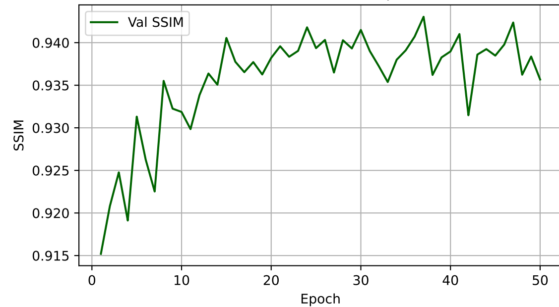
Validation SSIM over Epochs
