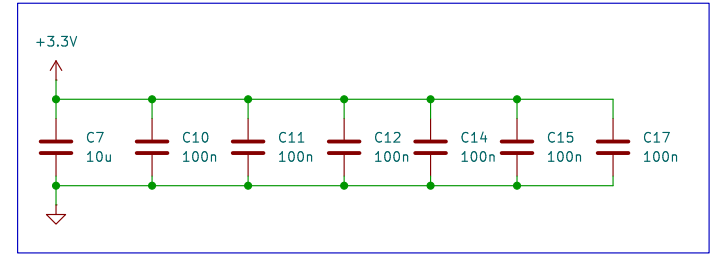
DECOUPLING CAPACITORS
