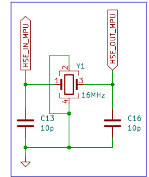
HIGH SPEED EXTERNAL CRYSTAL
