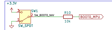
BOOT SWITCH
