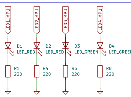
Status LEDs
