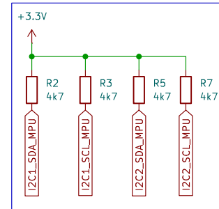
I2C Pullups
