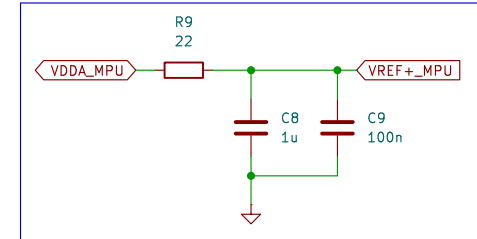
VREF+ FILTER
