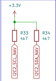
I2C Pullups
