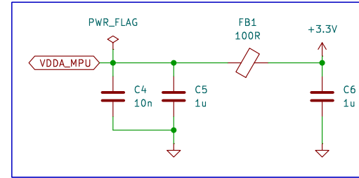
VDDA FILTER
