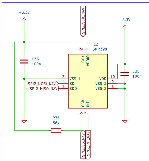
Pressure Sensor
