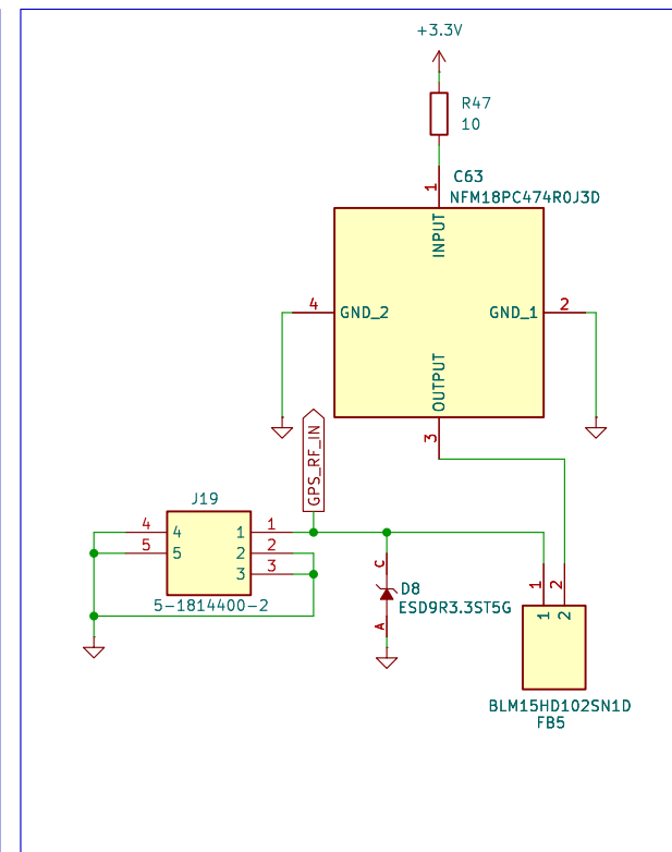
GNSS Antennaconnector
