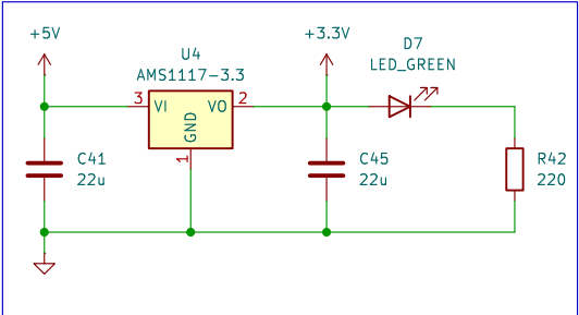
5V/3.3V Converter
