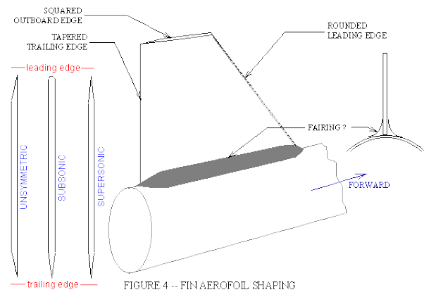
FIGURE 4 -- FIN AEROFOIL SHAPING
