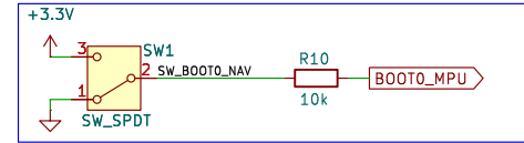
BOOT SWITCH
