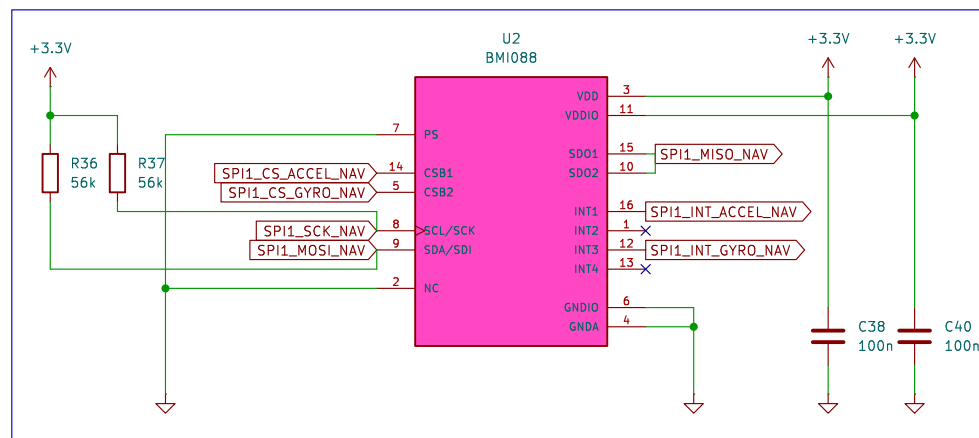
Primary IMU
