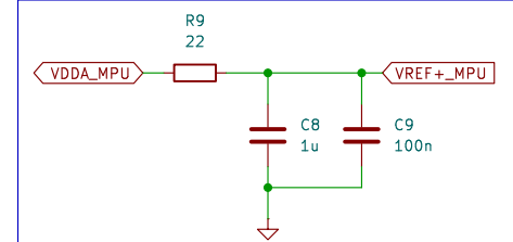
VREF+ FILTER
