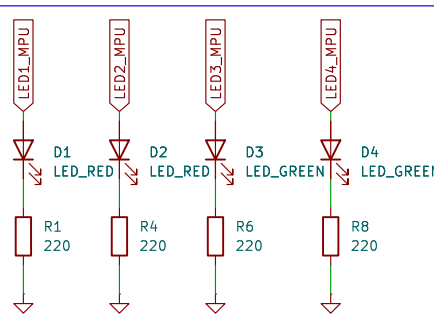
Status LEDs
