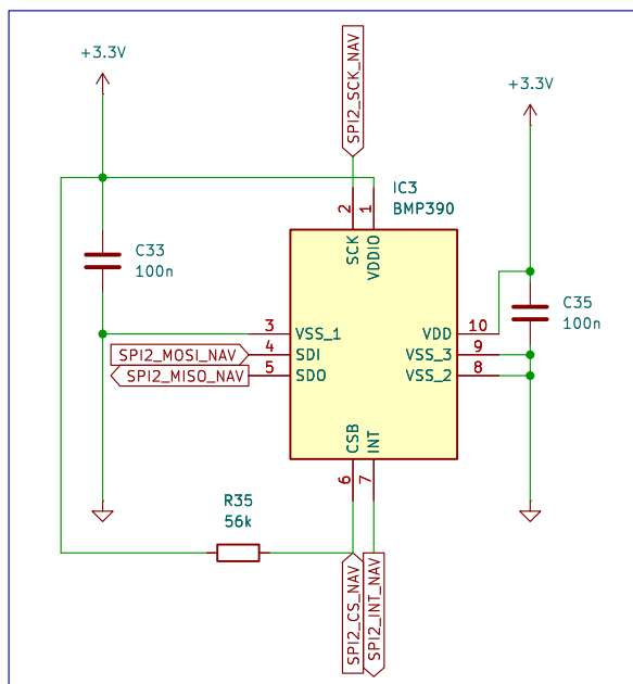
Pressure Sensor
