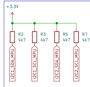
I2C Pullups
