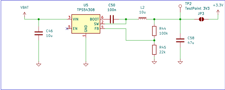
Buck Converter 8V/3V3
