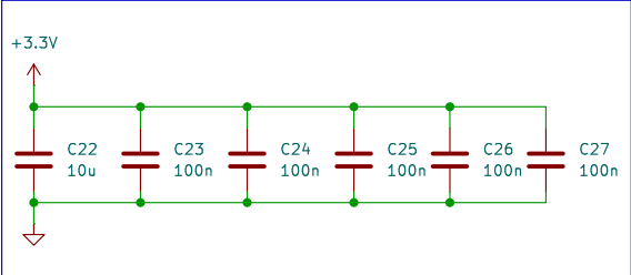
DECOUPLING CAPACITORS
