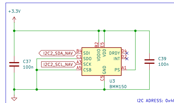
Magnetometer
