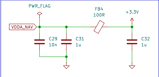
VDDA FILTER
