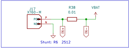
Battery Input and Current Sense Resistor
