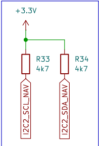
I2C Pullups
