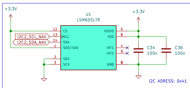
SECONDARY IMU
