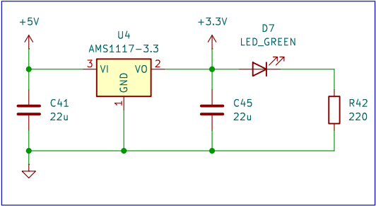
5V/3.3V Converter
