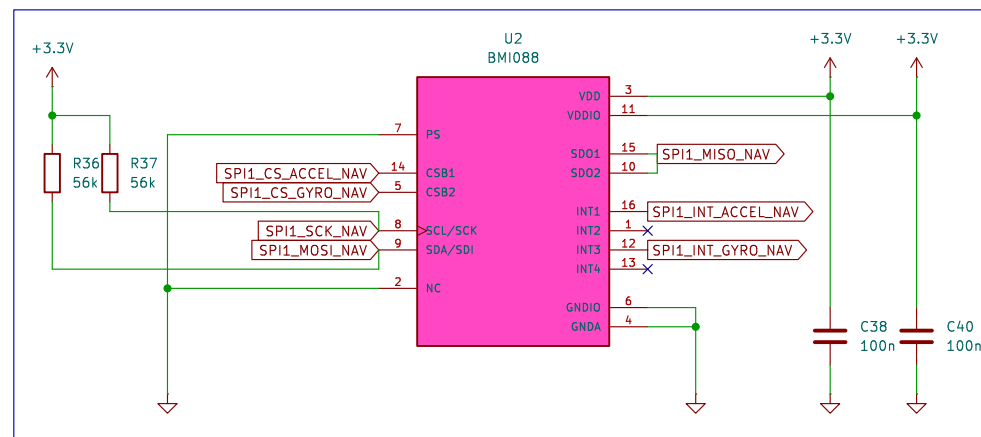
Primary IMU
