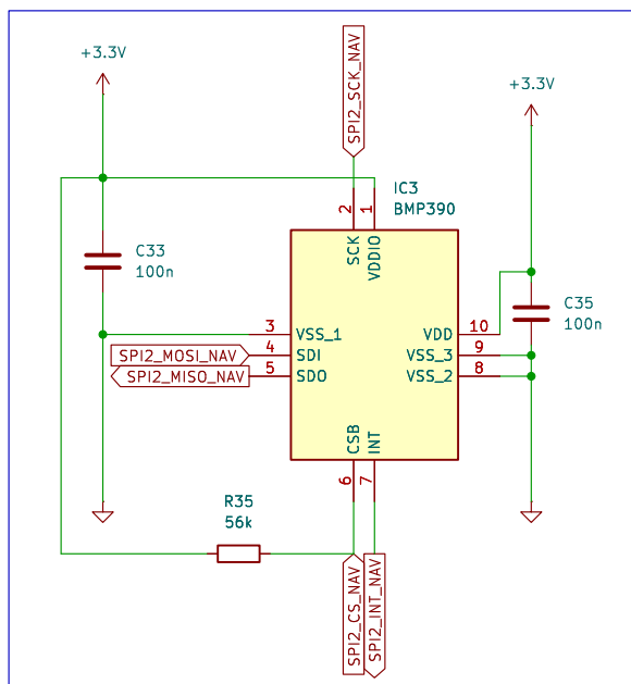
Pressure Sensor
