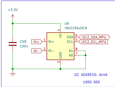
Voltage & Current Sensing
