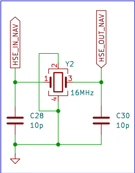
HIGH SPEED EXTERNAL CRYSTAL
