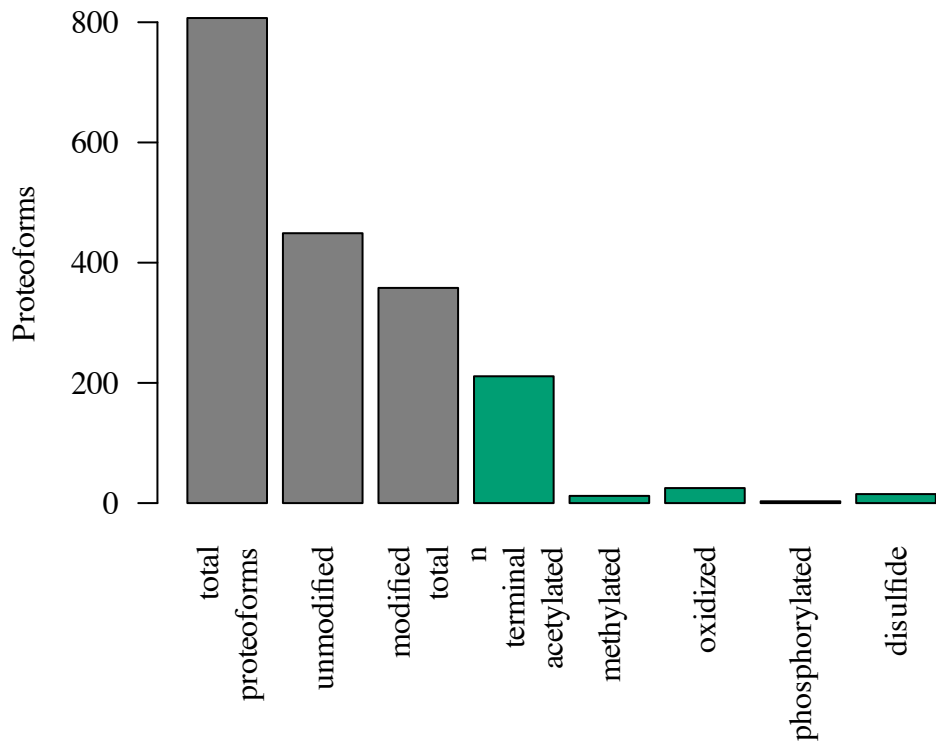
PTM inventory
