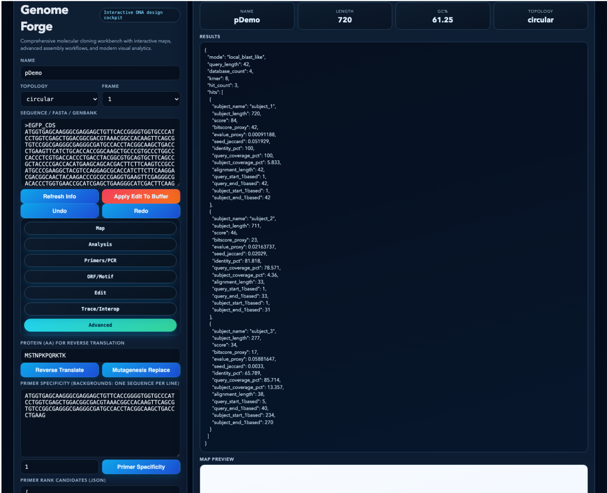
Figure 27. BLAST-like identity search workflow. Real UI screenshot from the local similarity-search case using the tutorial panel of EGFP, mCherry, lacZ, and BRAF. This is the kind of view you use to ask where an unknown sequence most plausibly came from.
