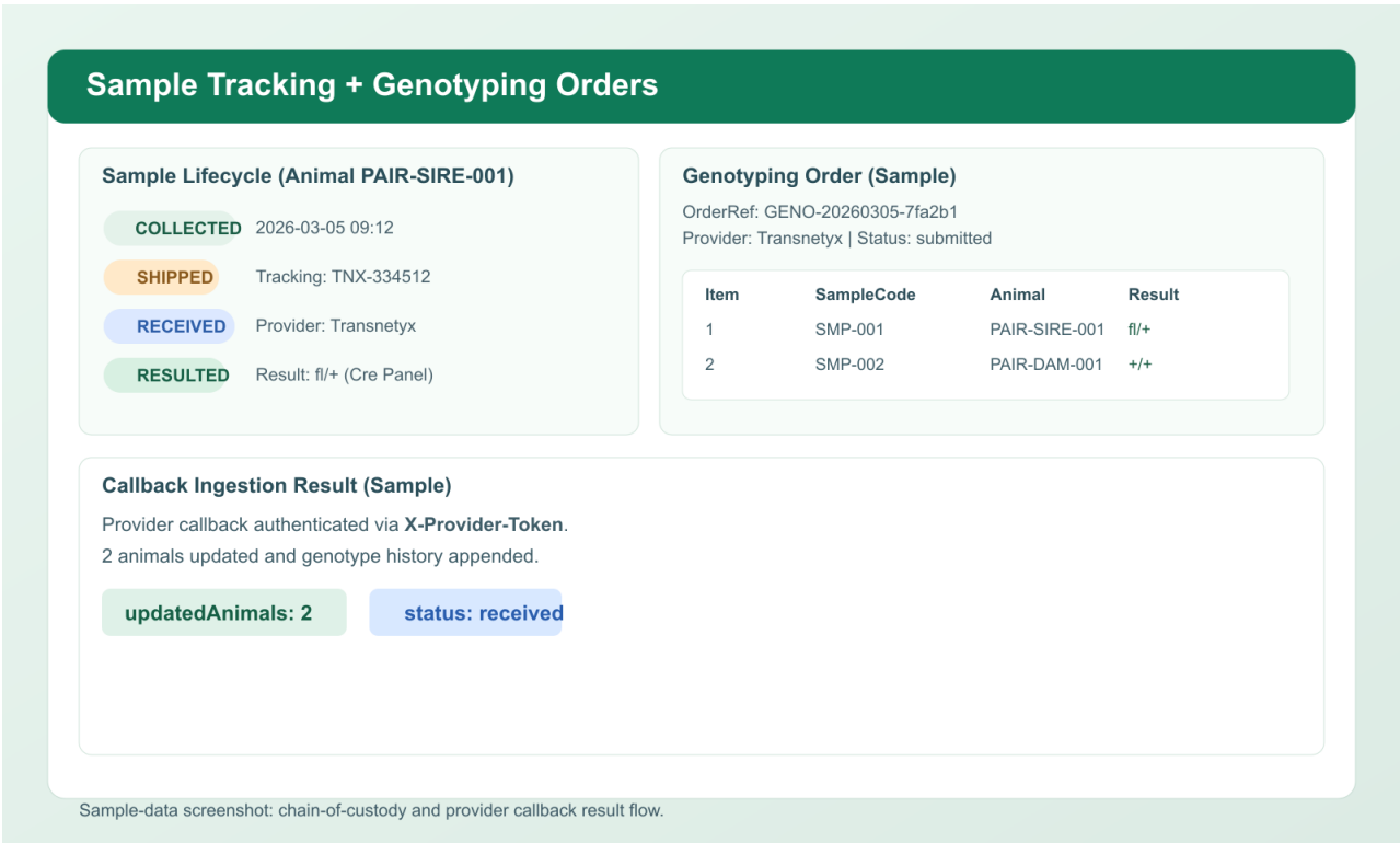
Figure 5: Sample chain-of-custody and genotyping result workflow
