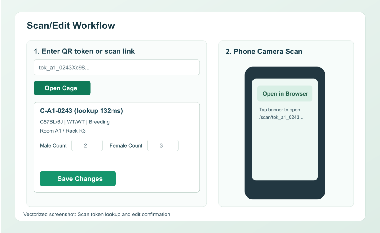
Figure 2: Phone scan flow from printed QR to cage browser view
